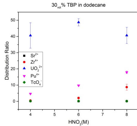
Fig. 3: Distribution ratios of U, Pu and fission products using 30Vol% TBP in dodecane as extractant.
