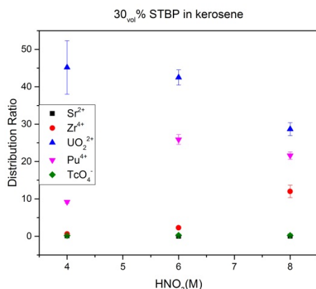
Fig. 4: Distribution ratios of U, Pu and fission products as 30 vol % STBP in kerosene.
