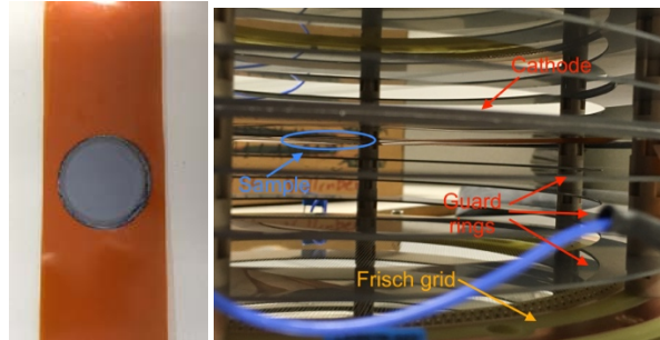
Fig. 3: Left: \text{Ta}_2\text{O}_5 glued on a 125 \mu\text{m} kapton support. Right: picture of the assembled detector with the target inside, parallel to the detector.
