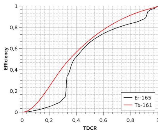
Fig. 2: Calculated efficiency vs. TDCR curves for Tb-161 and Er-165. Tb-161 is beta emitter with some contribution of low-energy gamma-rays and Er-165 is electron capture decaying radionuclide with multiple energy groups of Auger electrons and X-rays.
