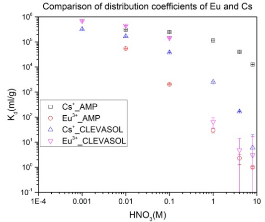
Fig. 1: Distribution coefficients of Eu and Cs on AMP and CLEVASOL.
