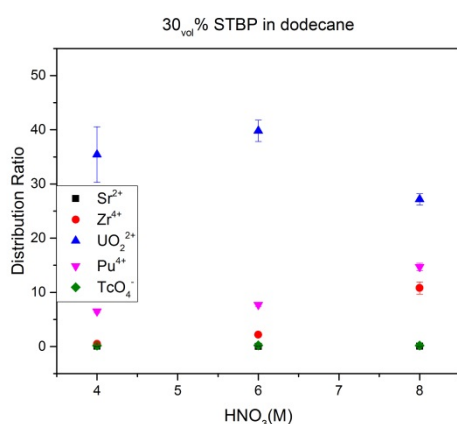
Fig. 5: Distribution ratios of U, Pu and fission products as 30 vol % STBP in dodecane.
