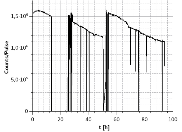
Fig. 2: Example irradiation history of a single UCN activation with multiple missed pulses, a large shutdown around 20 h, continuously dropping UCN intensity and an increase after a “conditioning procedure” which regains the solid D_2 performance, done at approx. 55 h (after ~5100 mC proton charge on target).
