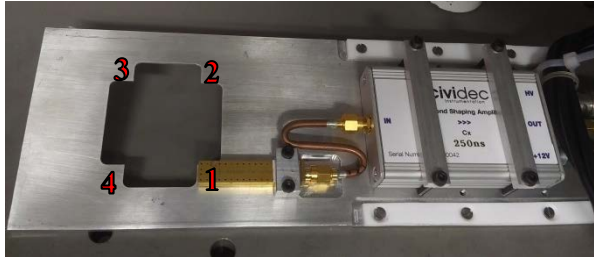
Fig. 4: The setup for activation at ICON with attached neutron detector and preamplifier. The opening enables passing of the majority of the beam. The samples are mounted at the corners of the opening, marked as positions 1-4.
