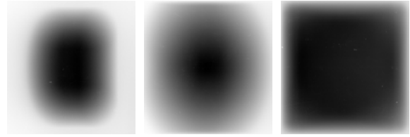
Fig. 5: 2D neutron beam profiles recorded at ICON beam port with 20 mm (left), 40 mm (center) and 80 mm (right) aperture.
