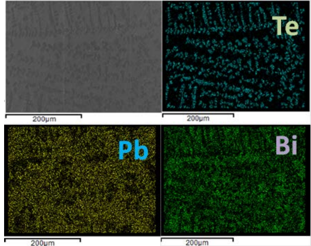
Fig. 2: Polished surface of the sample cross-section of LBE with 10% Te processed at 850 °C and rapidly solidified. SEM-Mag.: 149X / Mapping.
