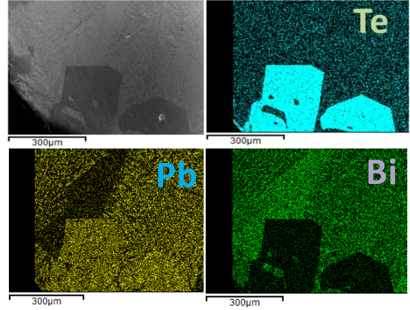
Fig. 1: Polished surface of the sample cross-section of LBE with 10% Te processed at 850 °C and slowly cooled to RT. SEM-Mag.: 149X / Mapping.
