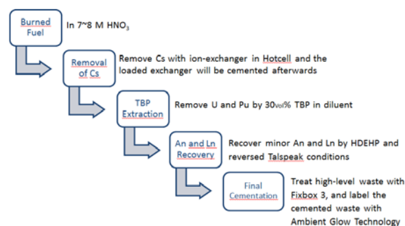
Fig. 2: Flow scheme of the waste conditioning.
