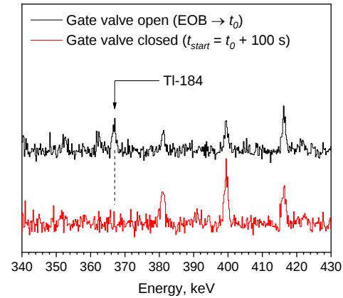
Fig. 4: Verification measurement of ^{184}\text{Tl} retained in the charcoal trap (spectra offset for convenience); gate valve open (top, black: t_{\text{live}} = 913\ \text{s} ) and another measurement started 100 s after the gate valve was closed (bottom, red: t_{\text{live}} = 900\ \text{s} ).
