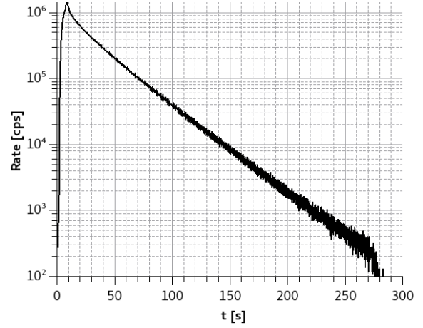
Fig. 1: Time profile of UCN delivery to a beam port after a proton pulse. Pulse period was 300 s.
