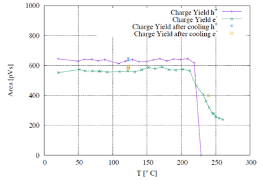
Fig. 2: The average area of the charge yield is plotted as function of the temperature. The purple line and blue crosses indicate the transmission of holes ( h^+ ) through the diamond bulk, whereas the green line and yellow squares show the conduction of electrons ( e^- ).
