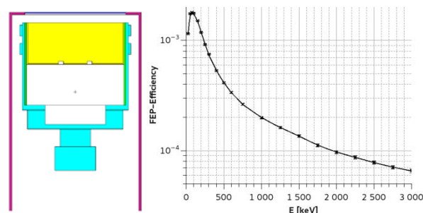
Fig. 1: Cut through MCNP model of a Canberra BEGe-Type detector including exact dimensions on germanium crystal, the endcap and the crystal holder (left), MCNP-calculated FEP efficiency curve for a point-like source in aluminum sample holder in 33 cm distance (right).
