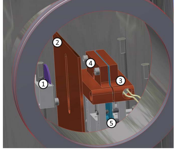
Fig. 1: Schematic of the setup used for the studies of a diamond-based detector in high temperature environments, with 1 being the ^{241}\text{Am} -source, 2 a copper heat shield with collimator to minimize the heat load of the ^{241}\text{Am} -source, 3 the copper heating block with inserted heating cartridge, 4 front copper heating block with collimator and 5 the PCB with the detector.
