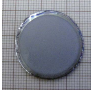
Fig. 2: \text{Ta}_2\text{O}_5 (central bluish-grey area) obtained by anodic oxidation of tantalum.
