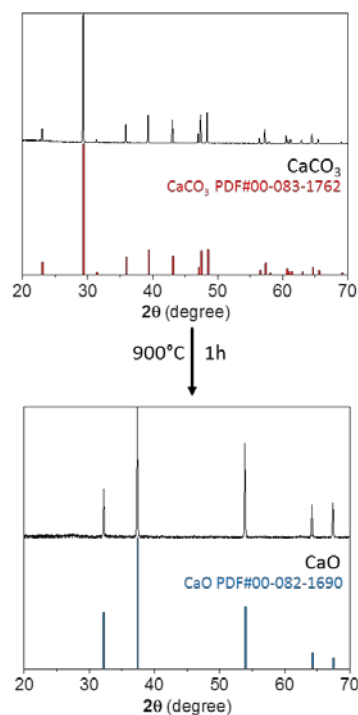
Fig. 3: X-ray diffraction patterns obtained from as purchased \text{CaCO}_3 (above) and CaO, obtained after thermal decomposition (below).
