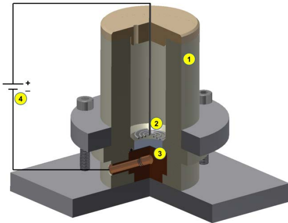
Fig. 1: Three dimensions schema of electrolytic cell.
