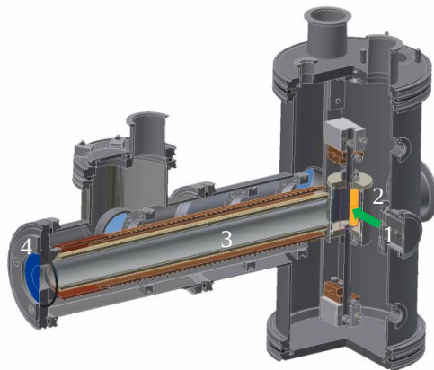
Fig. 3: Schematic of the optimized IVAC. The quartz column was enlarged to a diameter of 3 cm and a length of 40 cm, with 1 being the ^{252}\text{Cf} -source (the green arrow symbolizes the recoil path of the FPs to the HC), 2 the HCV with a hot Hf-foil, 3 the new and bigger isothermal quartz column, and 4 the detection flange, where a \gamma -detector can be placed in front of the opening of the column end to measure the FP's arriving there.
