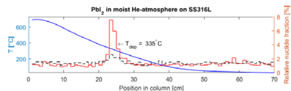
Fig. 3: Histograms of the radionuclide depositions observed in the experiments with SS316L and dry/moist helium with samples consisting of (a) \text{BiI}_3 (b) \text{BiI} (c) \text{PbI}_2 as well as the temperature at the point of deposition. The red solid line depicts the measured distribution of ^{126}\text{I} , the dashed lines are ^{206}\text{Bi} (blue) and ^{203}\text{Pb} (black). The solid blue line is the applied temperature gradient.
