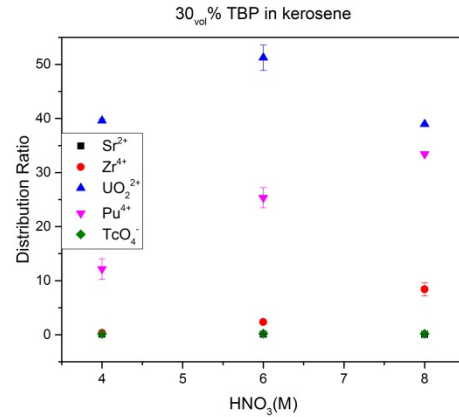
Fig. 2: Distribution ratios of U, Pu and fission products using 30Vol% TBP in kerosene as extractant.
