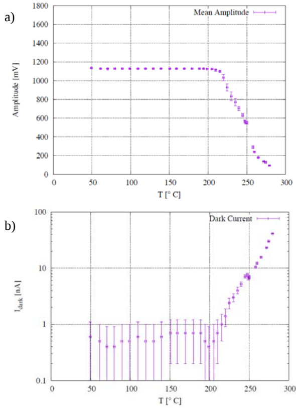
Fig. 3: a) Signal amplitude as function of temperature. b) Dark current as function of temperature. Both measurements were performed simultaneously.
