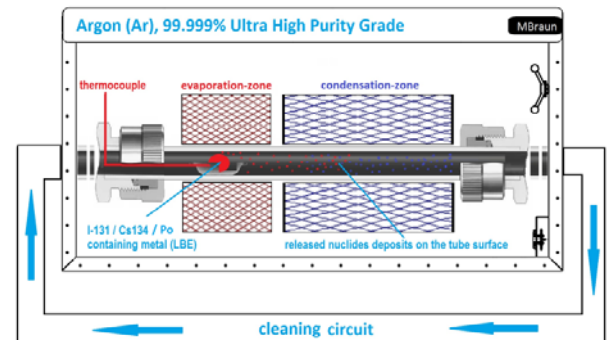
Fig. 1: Schematic outline of the transpiration setup.
