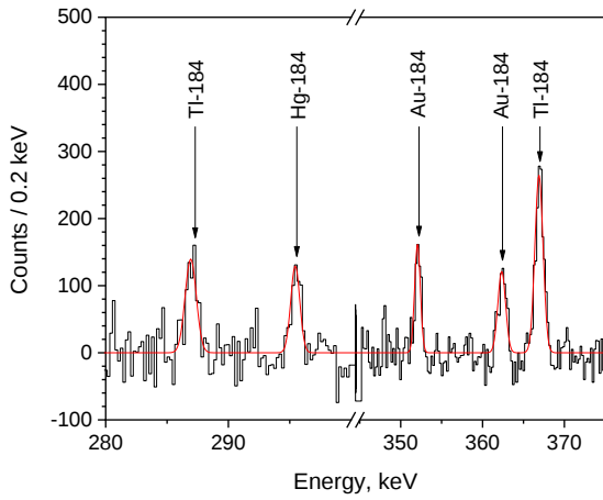
Fig. 3: Excerpt of a background subtracted \gamma -spectrum (black line) and the corresponding fit (red line), recorded during the collection for a direct catch measurement ( t_{\text{live}} = 3600\ \text{s} ); the two main \gamma -lines of ^{184}\text{Tl} are clearly visible.
