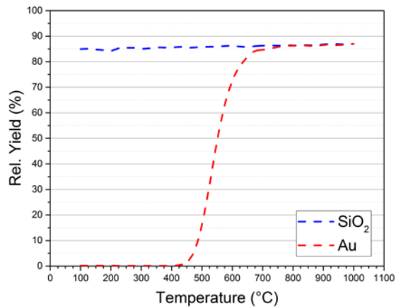
Fig. 2: The breakthrough curves obtained by MCS for the IVAC of ^{284}\text{Nh} on \text{SiO}_2 (blue) and Au (red). The maximum yield achieved with a column specific yield above, is 87% for both surfaces.
