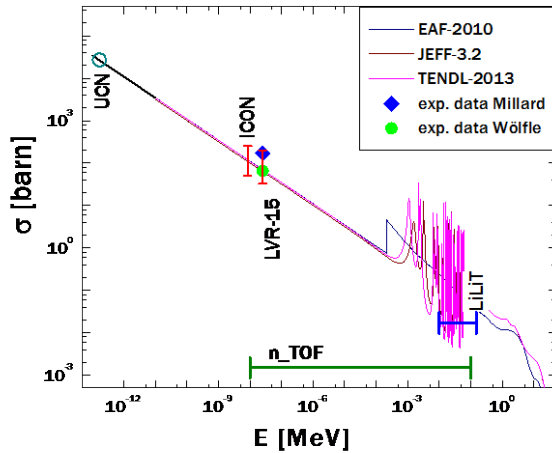
Fig. 1: Neutron capture cross-section of Mn-53 together with marked energy regions of the planned experiments. Experimental data and calculated excitation functions are referenced in the inset.
