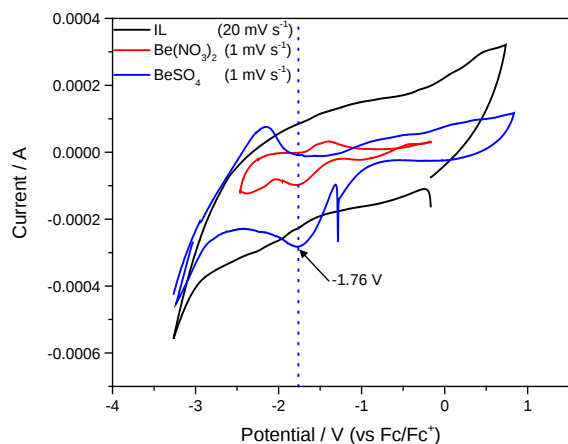
Fig. 2: CVs of pure [BMPi][TFSI], black curve, \text{Be}(\text{NO}_3)_2 and \text{BeSO}_4 in [BMPi][TFSI], red curve and blue curve, respectively.
