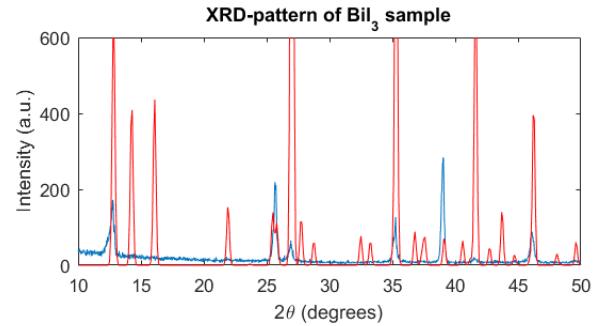
Fig. 2: XRD-pattern of metallic plate like crystals (blue) overlaid with reference XRD-pattern of BiI 3 (red).
