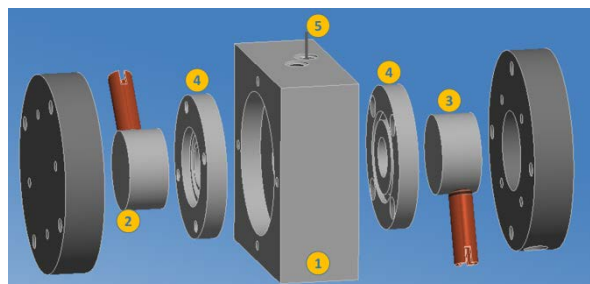
Fig. 1: Three electrodes electrodeposition cell.
