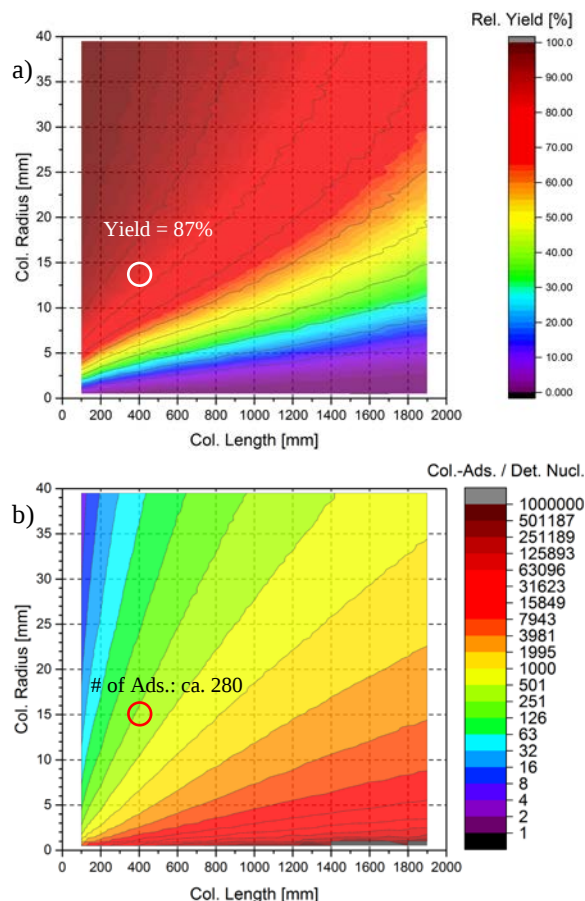
Fig. 1: a) The yield is plotted as function of radius and length of the column. The curving of the lines can be explained by the fact that the hot catcher volume (HCV) was included in the simulations and thus a more efficient transport between the HCV and the isothermal column is obtained at larger radii of the column. b) The number of adsorptions on the column per detected nuclide is plotted as function of radius and length of the column. Here, the adsorptions within the HCV are neglected.
