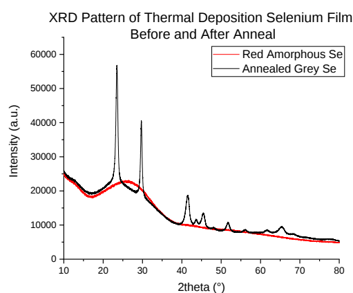
Fig. 5: XRD signal of TVD selenium film on glass slide, before and after heat treatment.
