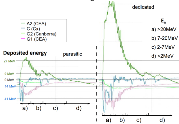
Fig. 4: Example of the output coming from different detector electrodes, each coupled to a different preamplifier.
