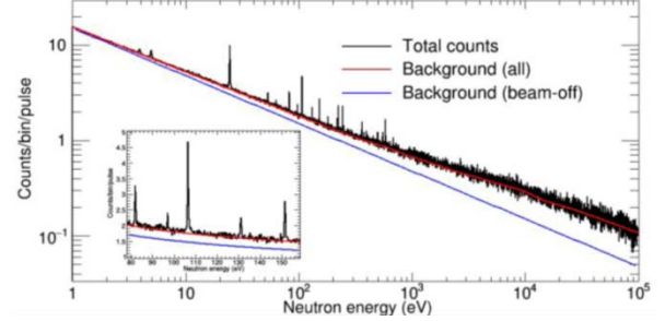
Fig. 1: Neutron energy distribution of the ^{171}\text{Tm} and background measurements at the CERN n_TOF facility, with ^{171}\text{Tm} resonances showing up above the background level.
