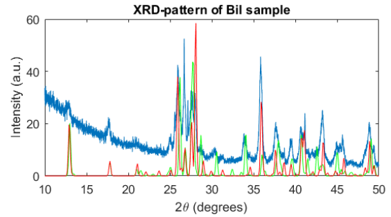
Fig. 1: XRD pattern of metallic grey sintered powder sample (blue) overlaid with reference XRD-pattern of \alpha -BiI (green) and \beta -BiI (red).
