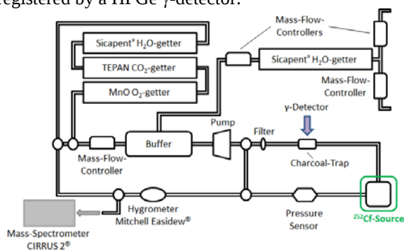
Fig. 1: Schematic representation of the model-system used for studying the formation of metal carbonyl complexes under single atom chemistry conditions.
