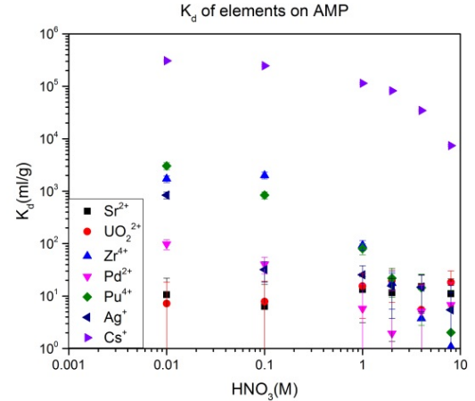
Fig. 2: Distribution coefficients of different elements on AMP.
