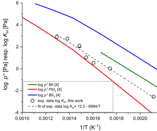
Fig. 3: Comparison of Henry constants of 131 I in LBE obtained in this work and the vapor pressures of pure PbI 2 , BiI and BiI 3 .
