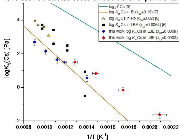
Fig. 2: Results of transpiration experiments using two specimens with different mass and mole fractions of Cs in comparison with literature data [6-9].
