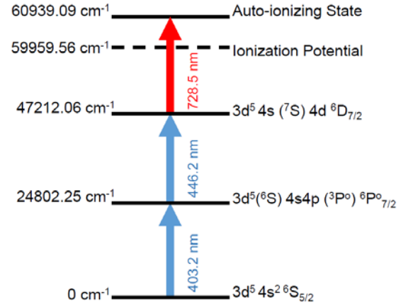
Fig. 1: Laser excitation scheme for Mn. Starting from the atomic ground state Mn atoms are resonantly ionized via two intermediate bound states into an auto-ionizing state by pulsed laser radiation.
