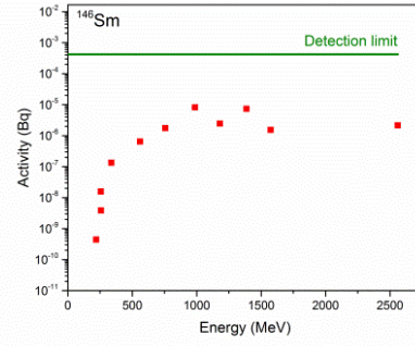
Fig. 5: Theoretical ^{146}\text{Sm} activities in proton-irradiated Ta targets (green line shows the detection limit of the 450 mm 2 \alpha -PIPS detector).
