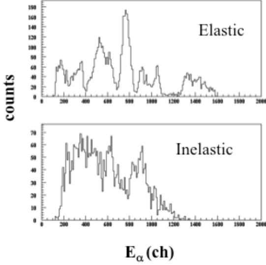
Fig. 2: Residual energy \alpha -particle spectra at \theta_{\text{lab}}=0^\circ . Top: elastic scattering events. Bottom: inelastic scattering events.
