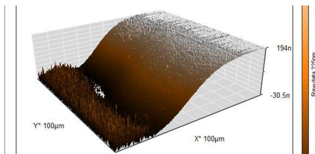
Fig. 2: Atomic force microscopy image of the \alpha -detector quartz-selenium interface. The deposited selenium (right, elevated plateau) shows a very smooth surface with a thickness of approx. 225 nm.
