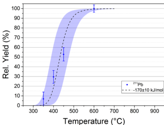
Fig. 1: Determination of the \Delta H_{\text{ads}} of Pb on quartz by comparing the obtained experimental (blue symbols) values to simulated data (black dotted lines and blue shaded area).
