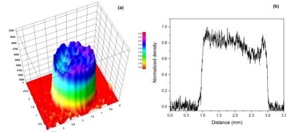
Fig. 4 : After molecular plating (with spiral anode and ultrasonic stirrer), RI 3D graph (a) and ^{153}\text{Gd} activity distribution (b).
