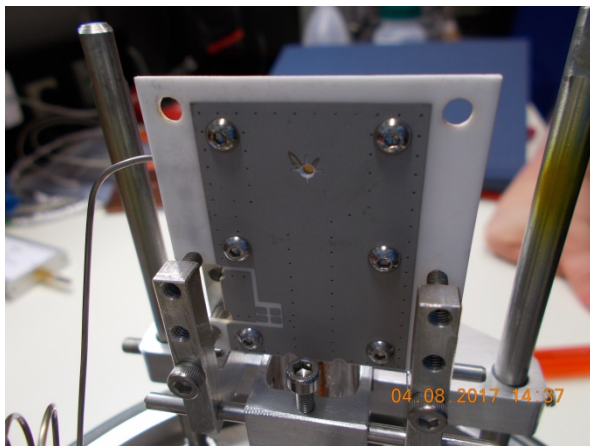
Fig. 4: The alumina PCB-structure containing the diamond-based sensor, mounted in the setup, without the heating cartridges; the type-K thermocouple can be seen on the left hand side.
