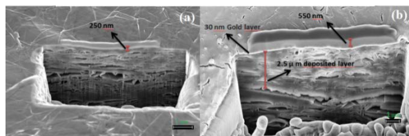
Fig. 2: Comparison of the SEM image of the carbon foil before (a) and after Gd deposition (b) with wedge angle prepared by FIB-milling perpendicular to the sample, showing the thickness of Gd deposited layer.
