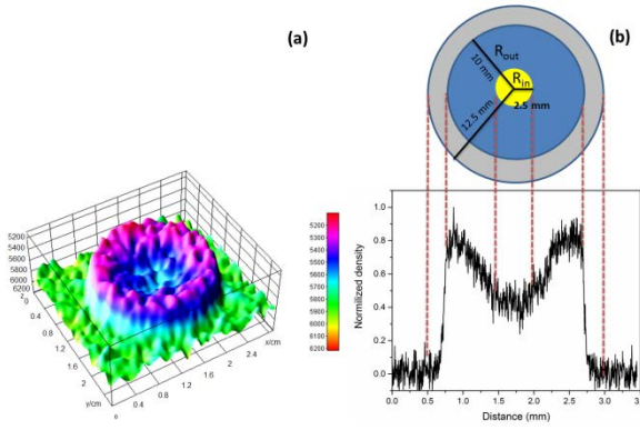
Fig. 3: After molecular plating (with spiral anode), RI 3D graph (a) and ^{153}\text{Gd} activity distribution (b).
