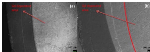
Fig. 1: SEM image of the edge of the Gd deposited carbon layer before (deposited area: 3.14 \text{ cm}^2 ) (a) and after gold coating (b) (gold coated area: 3.80 \text{ cm}^2 ).
