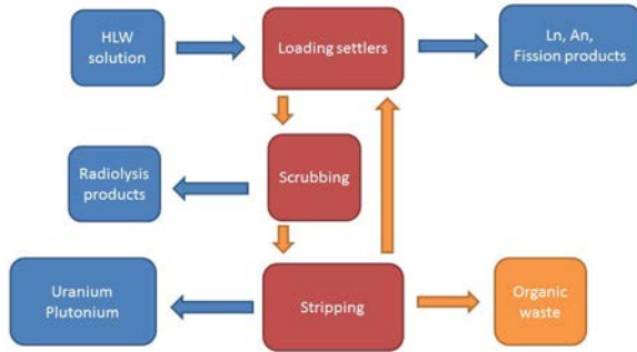
Fig. 1: Schematics of the solvent extraction facility for extraction of actinides and lanthanides from nuclear fuel solutions. Organic fraction is marked in orange, aqueous phases in blue.
