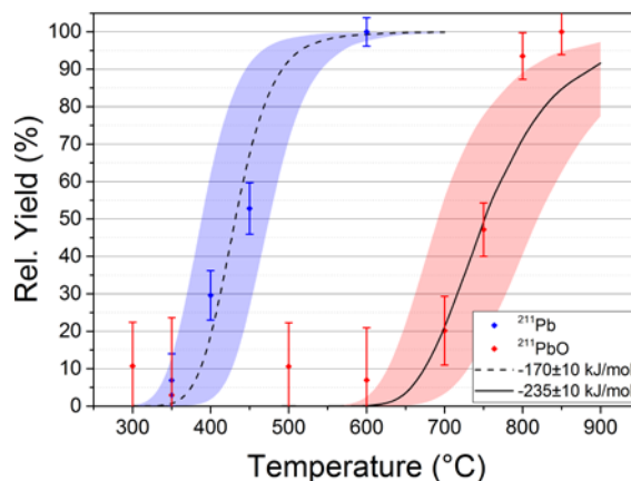
Fig. 2: The two observed species of elemental ^{211}\text{Pb} and the compound ^{211}\text{PbO} , with their determined adsorption enthalpies (Data of ^{211}\text{PbO} adapted from [4]).
