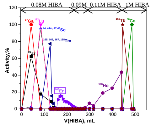
Fig. 1: Elution profile of Er separation from the target material and formed impurities
