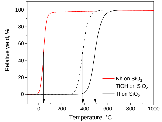
Fig. 2: Monte-Carlo simulations, using the microscopic kinetic model at zero surface coverage [4], for Nh (red line, -\Delta H_{ads}^{SiO_2}(\text{Nh}) = 57.8 kJ/mol), TlOH (black dashed line, -\Delta H_{ads}^{SiO_2}(\text{TlOH}) = 134 \pm 5 kJ/mol), and Tl (black line, -\Delta H_{ads}^{SiO_2}(\text{Tl}) = 158.3 \pm 3 kJ/mol) on quartz and under consideration of all experimental parameters; the arrows indicate the temperature at a relative yield of 50%.
