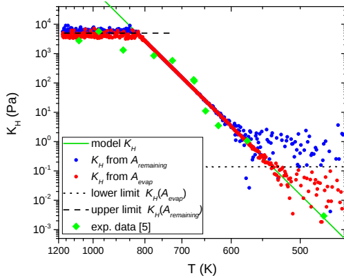
Fig. 1: Comparison of modelled Henry constant data and experimental data obtained from transpiration experiments (see text for detailed explanations).
