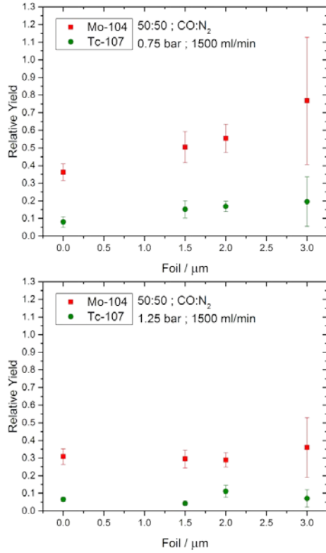
Fig. 2: Plot of the obtained relative yield (see text) of carbonyl complexes obtained for 50:50 mixtures of CO and N 2 and a gas flow rate of 1500 mL/min, different kinetic energies and two different pressures. Each measurement was repeated three times. The standard deviations, shown as error bars, were obtained by error propagation.
