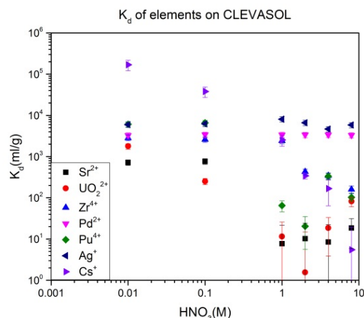
Fig. 3: Distribution coefficients of different elements on CLEVASOL.
