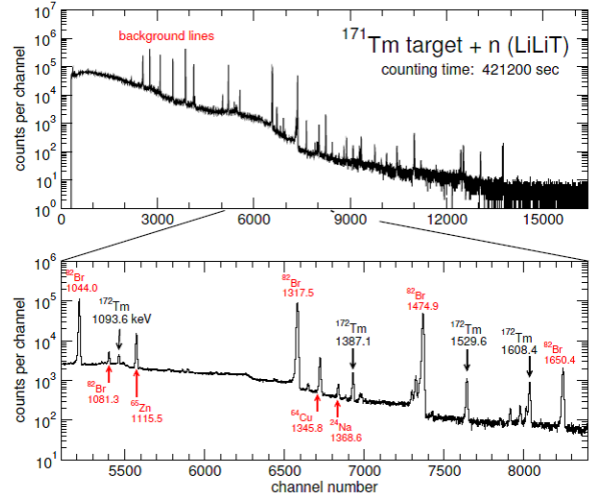
Fig. 2: Decay spectrum after activation of the ^{171}\text{Tm} target at LiLiT: four decay lines from ^{172}\text{Tm} have been used to extract the MACS values.
