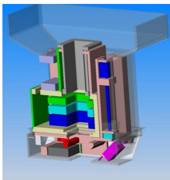
Figure 2 shows the cross section of the Gantry 2 nozzle. The light blue and green box are the dose measurement monitor and the dark blue is the position sensitive monitor.
