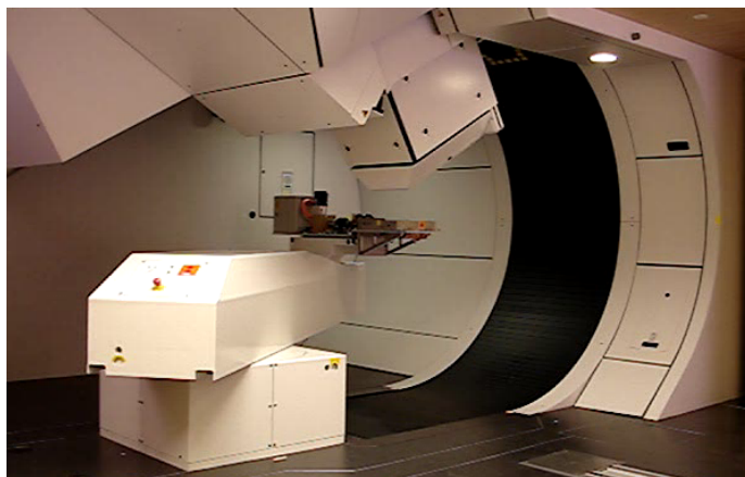
Figure 1 shows the Gantry 2 with a replica of the nozzle position detector to execute some quality assurance measurements.
