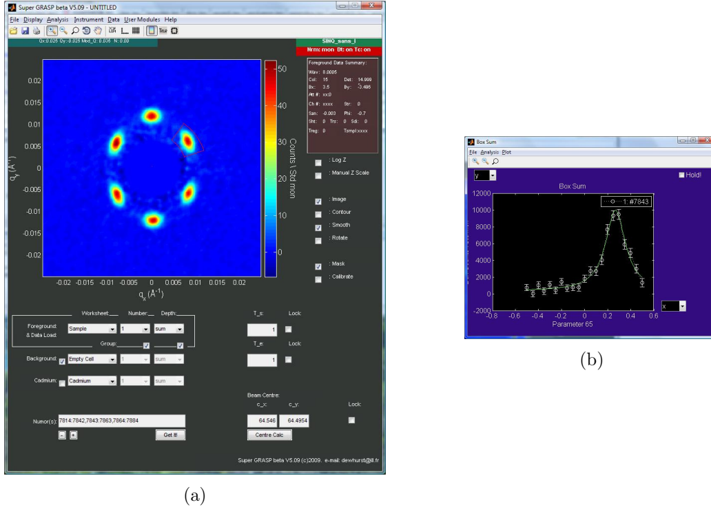
Figure 6: (a) Image capture of the front-end of the GRASP software (version 5.09). SANS data over multiple rocking curves is loaded, showing all the first-order Bragg spots in a single image. A sector box is defined on the detector over area occupied by the upper right Bragg spot. (b) Image capture of a rocking curve plot output by the GRASP software, and fit with a suitable lineshape function. The horizontal axis is in units of degrees of rotation angle of the reciprocal lattice about the vertical axis, where zero corresponds to the straight through position. The vertical axis is in units of total counts within the sector box per standard monitor.
