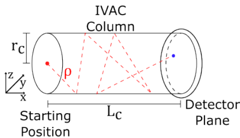
Figure 1: Isothermal vacuum chromatography setup with indicated size parameters and an example trajectory (dashed red line). The length of the first flight step \rho is indicated; the blue point marks the final adsorption position on the detector.
