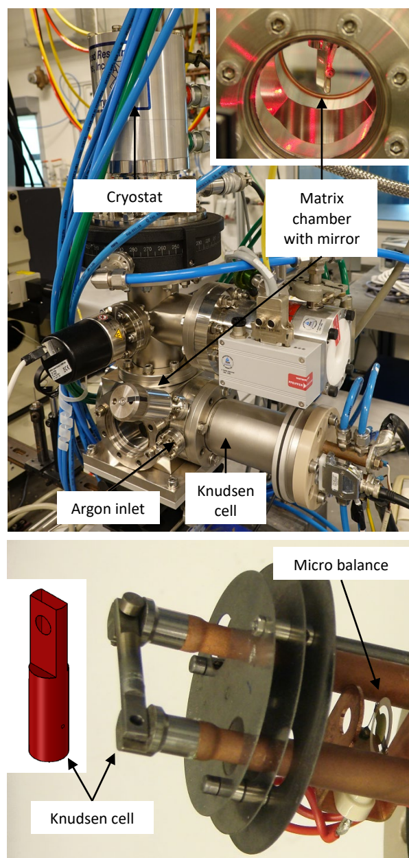
Figure 1: Top picture: Image of the matrix isolation setup, which consists of the main chamber, a side chamber containing the Knudsen cell, as well as a He-cooled cryostat. (Insert: Main chamber with the Ir-coated mirror) Bottom picture: Knudsen cell fixed between the heating elements. The quartz crystal microbalance is located behind the heat shield. (insert: schematic of the Knudsen cell with one hole visible)
