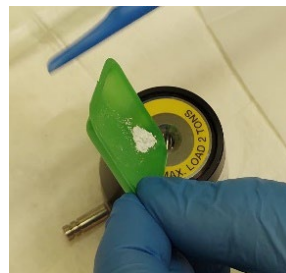
Figure 2: Filling of powder into pressing chamber.
