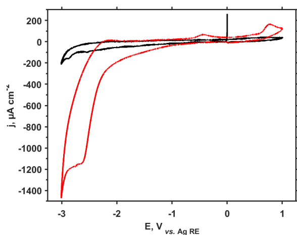
Figure 2: First cycle of the CV of pure [BMP][TFSI] (black) and of Tb in [BMP][TFSI] (red), both recorded using a Au WE at a scan rate of 50 \text{ mV s}^{-1} and at room temperature.
