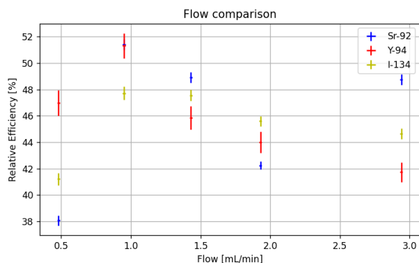
Figure 3: Evolution of the relative efficiency with the solvent flow at the inlet of the degasser unit.
