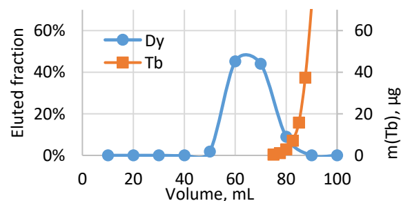
Figure 2: Reproducible elution profiles of 5 \mu\text{g} Dy and 40 mg Tb on Sykam Resin column with pump rate 0.7 mL/min and eluent \alpha -HIBA 0.11 M.
