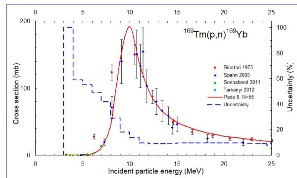
Figure 1: Experimental ^{169}\text{Tm}(p,n)^{169}\text{Yb} cross section data including Pade fit (Figure is taken from ref 3).
