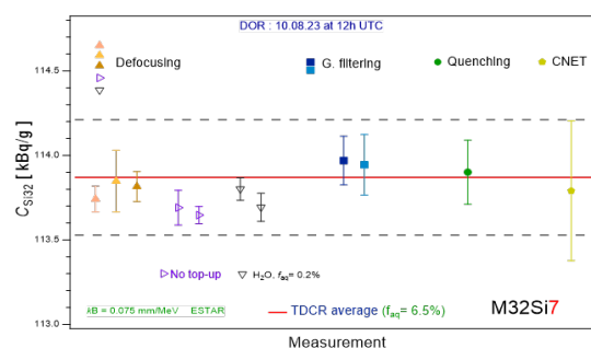
Figure 1: TDCR and CNET activity measurements of the M32Si7 solution. The red line is the arithmetic average of all TDCR measurements of samples with HCl 0.5 M top-up ( f_{aq} = 6.5\% ).
