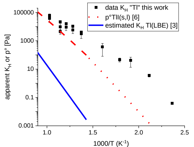
Figure 3: apparent Henry constant of Tl in non-reduced LBE prepared from Pb and Bi with 99.9999% purity, containing iodine as impurity with a mole fraction of ca. 6 \times 10^{-4} , measured in purified helium gas at a flow of 100 ml/min.
