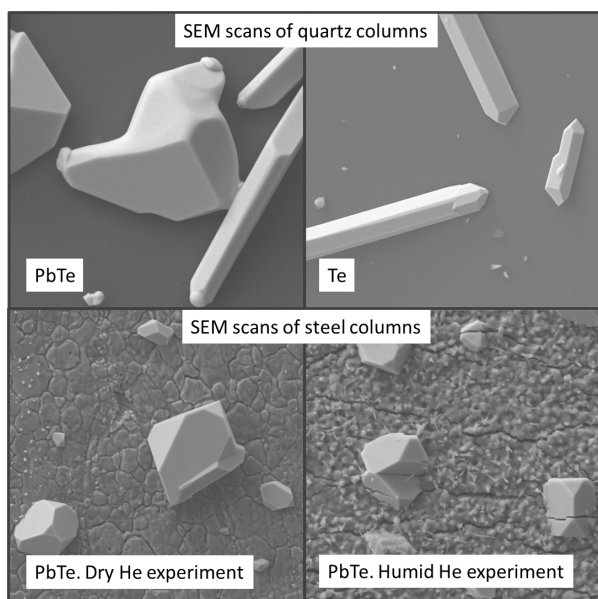
Figure 1. SEM images of depositions found in quartz and steel columns.
