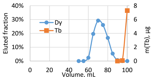
Figure 3: Reproducible elution profiles of 5 µg Dy and 40 mg Tb on Sykam Resin column with pump rate 0.6 mL/min and 0.11 M \alpha -HIBA as eluent.
