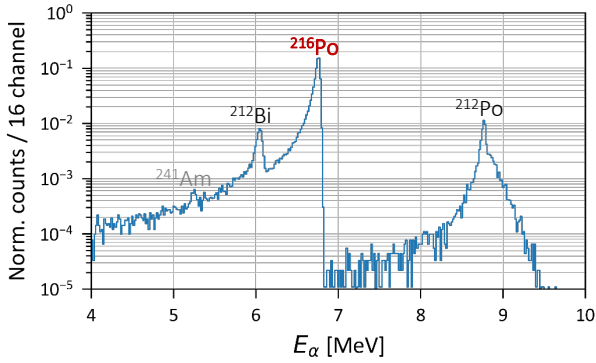
Figure 2: Example \alpha -spectrum of ^{216}\text{Po} and its daughter radionuclides ^{212}\text{Bi} and ^{212}\text{Po} (with large high-energy tailing due to ^{212}\text{Bi} + ^{212}\text{Po} pile-up events). The clear observation of ^{216}\text{Po} proves the successful transport of the short-lived species. ^{241}\text{Am} was used as a calibration source mounted on axis at the beginning of the thermalization chamber.
