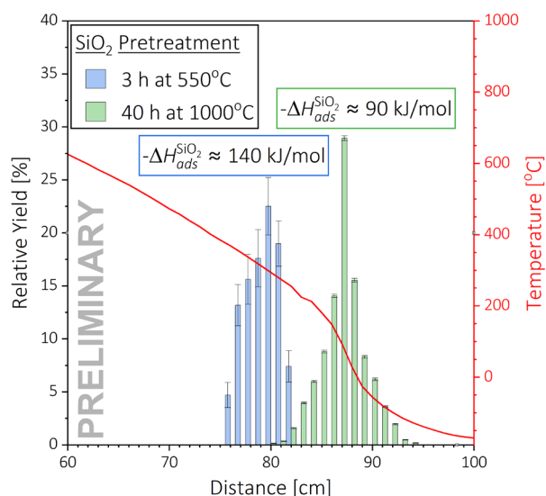
Figure 1: The preliminary internal chromatograms (blue and green bars; normalized to the associated individual total sum) resolved at 1 cm steps and the temperature profile (red line and right axis) as well as the preliminary negative adsorption enthalpies (color coded).
