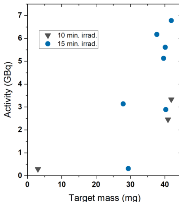
Figure 2: Activity of targets at EOB vs target mass ( ^{68}\text{Zn} ).
