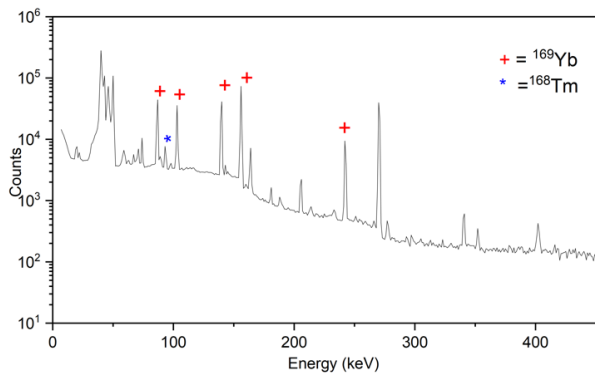
Figure 3: Gamma spectrum of proton-irradiated \text{Tm}_2\text{O}_3 target (counting time: 237404 s, SDD:1 m).
