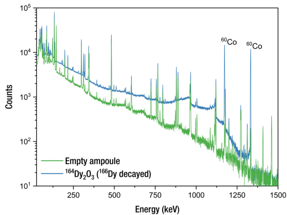
Figure 2: Comparison between the gamma spectra of Ampoule (2) after the complete decay of 166 Dy and the empty one.
