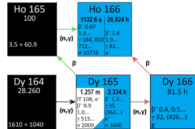
Figure 1: Karlsruhe nuclide chart showing the relevant radio-nuclides with the associated nuclear reactions and decay modes.
