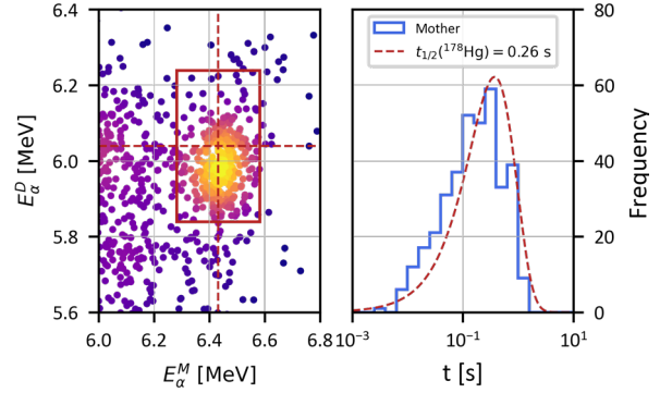
Figure 4: Example result of the recoil- \alpha - \alpha correlation analysis for ^{178}\text{Hg} with correlated events (left side) and the histogram of recoil- \alpha correlation times (right side), indicative for the half-life of the initially implanted mother radionuclide (red dashed line) [7]; the analysis confirms a successful production of short-lived ^{178}\text{Hg} (mother, M) in the irradiation of ^{144/147}\text{Sm} with a 210 MeV ^{36}\text{Ar} center-of-target ion beam energy. Chosen correlation window: E_\alpha^{\text{M}} = 6.43 \pm 0.10 MeV with 3 \cdot \tau^{\text{M}} = 1.13 s, E_\alpha^{\text{D}} = 5.980 \pm 0.125 MeV with 3 \cdot \tau^{\text{D}} = 3.86 s ( ^{174}\text{Pt} as daughter, D). The red lines in the left figure indicate the correlation windows for ^{178}\text{Hg} .
