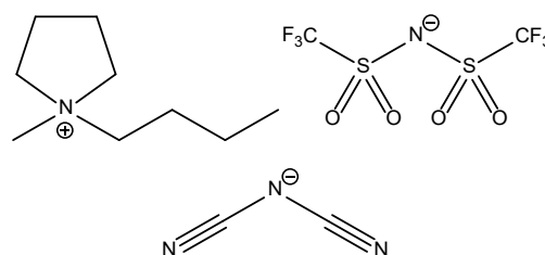
Figure 1: Structures of [BMP] + (top left), [TFSI] - (top right) and [DCA] - (bottom).
