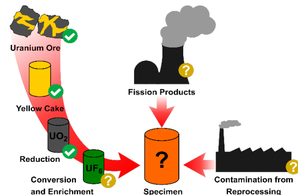
Figure 1: Today, the lanthanoid patterns in natural U materials are well-understood. However, the impact of enrichment, fuel irradiation and reprocessing remains unknown.
