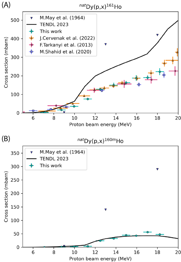
Figure 1: Comparison of experimental and theoretical production cross sections of (A) ^{161}\text{Ho} and (B) ^{160m}\text{Ho} in proton-irradiated ^{nat}\text{Dy}_2\text{O}_3 .
