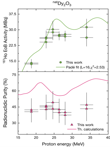
Figure 2: (Top) Comparison of our experimental data and calculations based on Padé approximant fitted using experimental and theoretical cross-section data of ^{nat}\text{Dy}_2\text{O}_3 . (Bottom) Radionuclidic purity results evaluated after a 5-hour cooling time. Irradiation conditions: I_p = 5 \mu\text{A} , t_{irr} = 5 \text{ min} , m_{tar} = 40 \text{ mg} .
