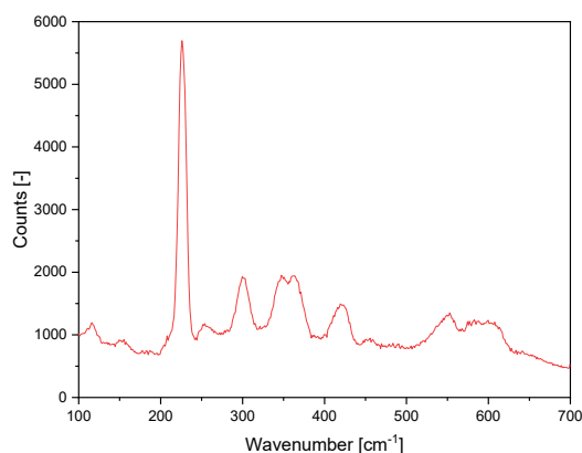
Figure 2: Raman spectrum of deposited S within the solid Ar matrix using an excitation wavelength of 532 nm.
