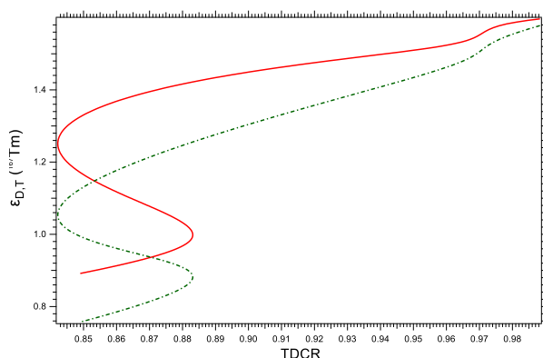
Figure 1: Variation of the ^{167}\text{Tm} double and triple detection efficiencies with the TDCR.
