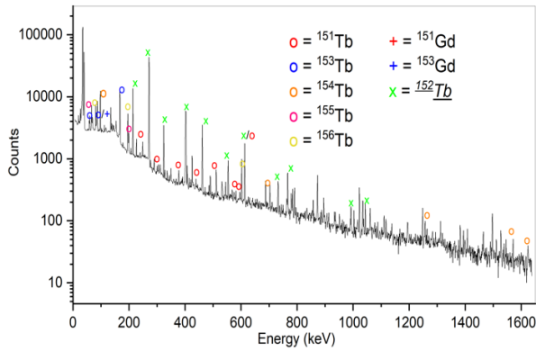
Figure 2: Gamma spectrum of proton-irradiated enriched ^{155}\text{Gd}_2\text{O}_3 target (counting time: 1917 s sample detector distance (SDD): 1 m).
