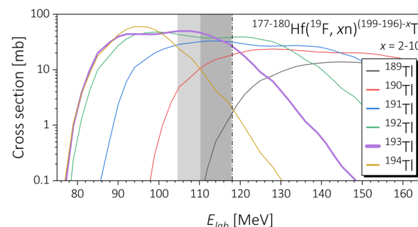
Figure 1: Cumulated cross sections for different Tl radioisotopes as calculated with the NRV [11] and normalized to the natural abundance of different Hf isotopes. The energy loss of the ^{19}\text{F}^{7+} ion beam (primary ion beam energy E_{\text{lab}} = 118 MeV, dot-dash black line) in the Be vacuum window + He cooling gas slit (dark shaded area) and the ^{180}\text{Hf} target (light shaded area) were calculated with SRIM [12].
