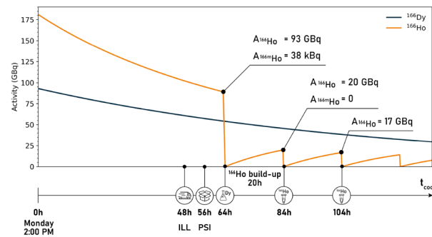
Figure 3: Qualitative trends of 166 Ho and 166 Dy following end of irradiation (EoI) considering a target mass of 650 \mu\text{g} 164 Dy 2 O 3 , irradiation time = 6 days, \Phi = 1.2\text{E}+15 \text{ cm}^{-2}\text{s}^{-1} . This plot displays a plausible production under the simplifying assumption of 100% separation yield at each step.
