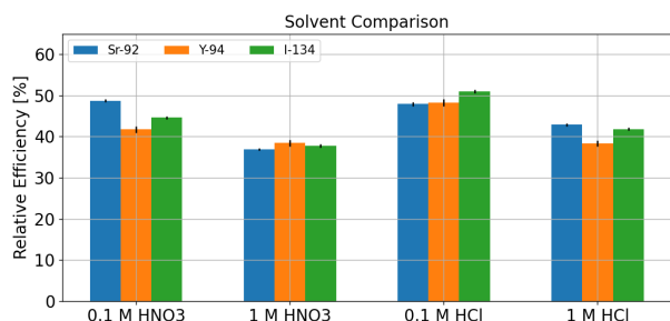
Figure 4: Variation of the relative efficiency as a function of the HCl and HNO 3 concentration.
