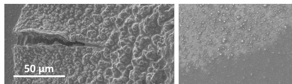
Figure 3: SEM images (same scale) of the Tb films as obtained by ED of Tb(III) from [BMP][TFSI] on a Au WE by applying a constant voltage of -1.8 \text{ V}_{\text{vs. Ag RE}} for 56 h (left) and 2 h (right) at RT.
