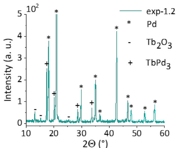
Figure 2: XRD patterns of exp-1.2 measured in reflection mode (MoK \alpha 1-radiation with \lambda = 0.70930 \text{ \AA} ). The three identified crystalline phases are (*) the Pd face-centered cubic crystal lattice, (+) the primitive cubic crystal structure of \text{TbPd}_3 , and (-) the body-centered cubic crystal lattice of \text{Tb}_2\text{O}_3 .
