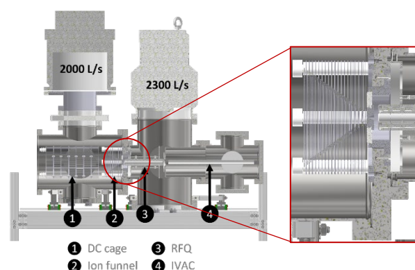
Figure 1: Developed BGC with thermalization chamber (DC cage, DC-RF ion funnel) connected to transfer chamber with the RFQ via a supersonic nozzle.
