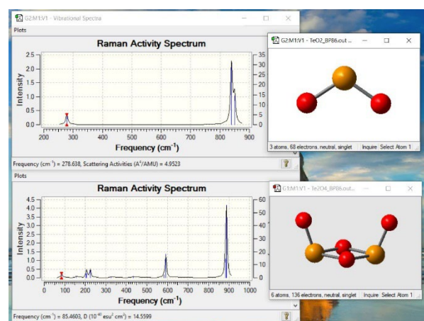
Figure 3: Calculated Raman spectrum of TeO 2 . The formation of both the monomer and the dimer seem plausible.
