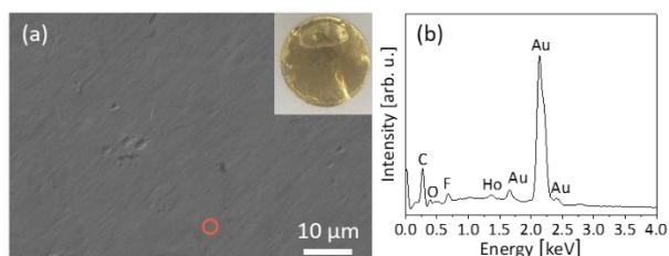
Figure 2: (a) the SEM image of the Au foil used as WE (insert) after applying -2.14 \text{ V}_{\text{vs. Fc}} for 48 hours to Ho-[BMP][TFSI] and (b) the EDX spectrum of a selected area (red circle in (a)).
