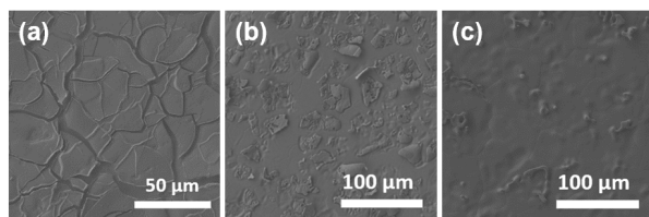
Figure 1: SEM images of central regions on (a) Sample 1, (b) Sample 2, and (c) Sample 3.
