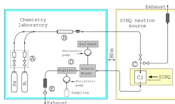
Figure 1: Scheme of the SINQ Gas-Jet system with the online dissolution; picture adapted from [3].
