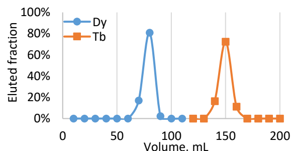
Figure 1: Reproducible elution profiles of Dy and Tb (both 5 \mu\text{g} ) on Sykam Resin column with 0.11 M \alpha -HIBA as eluent.
