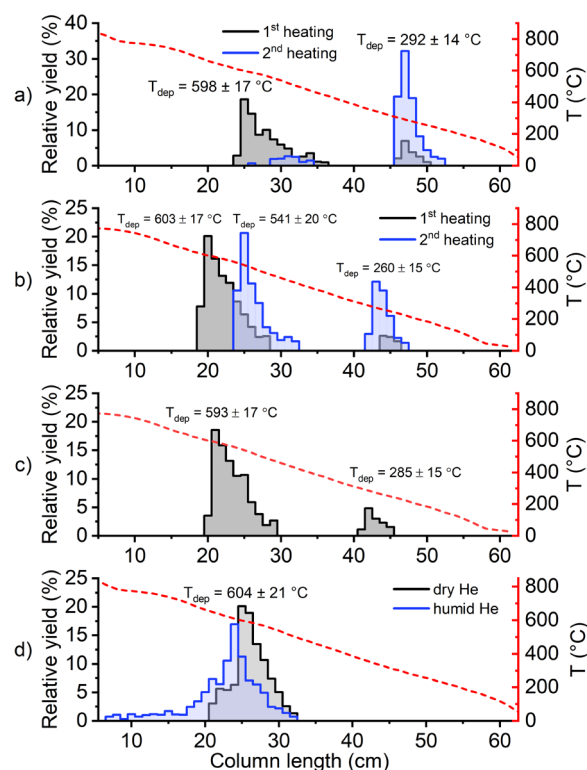
Figure 2. Thermosublimatograms of LBE-Te samples, where dashed line represents temperature gradient, and solid line shows distribution of Te. a) consecutive heatings in He with higher water impurity; b) consecutive heatings in He with lower water impurity; c) experiment with 10% admixture of \text{H}_2 to He; d) experiments in steel columns in dry and moist He atmospheres.
