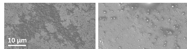
Figure 5: SEM images (same scale) of the Tb film as obtained by ED of Tb(III) from [BMP][TFSI] (left) and [BMP][DCA] (right) on a Au WE by applying a constant voltage of -1.8 \text{ V}_{\text{vs. Ag RE}} for 2 h at RT.
