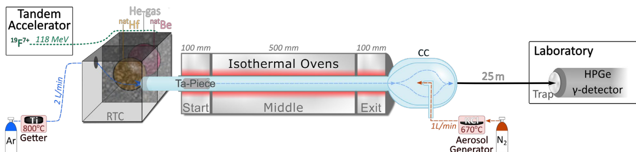
Figure 2: Schematic of ^{193\text{m}}\text{Tl} synthesis and subsequent chemistry setup at JAEA; see text for details.
