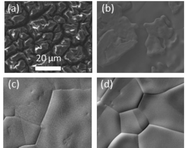
Figure 1: SEM images of (a) exp-1.1, (b) exp-1.2, (c) exp-1.3, and (d) exp-1.4. The scale, and therefore the resolution, is the same for all four SEM images.
