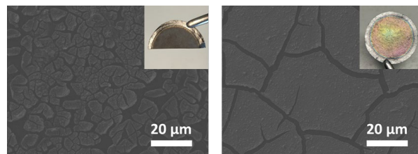
Figure 1: SEM images (magnification given at the bottom right) of the plated layer under anhydrous (left) and ambient condition (right); embedded are the digital images.
