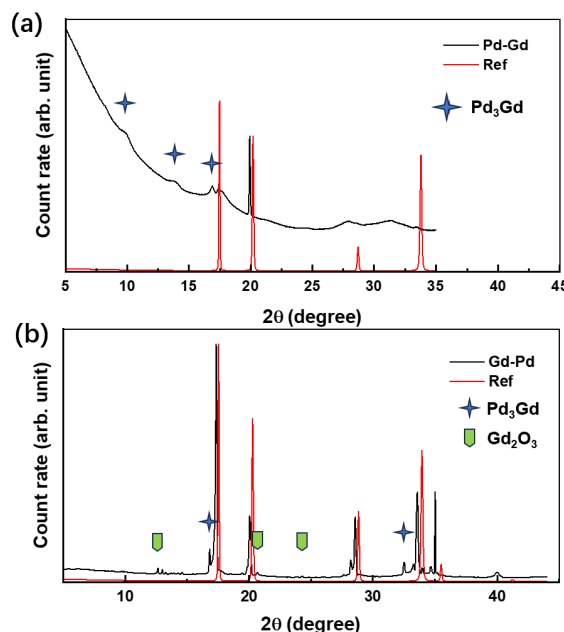
Figure 3: XRD pattern of selected regions in (a) Sample 6 and (b) Sample 5.
