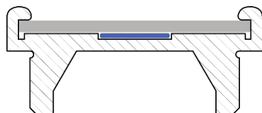
Figure 1: Cross cut through aluminium capsule containing the disc of target material at the centre. Proton beam enters the capsule from the top in this view.
