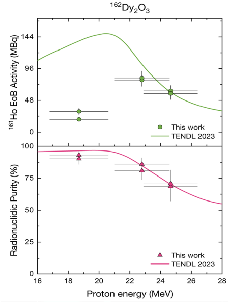
Figure 3: (Top) Comparison of our experimental data and calculations based on TENDL 2023 theoretical cross-section data of ^{162}\text{Dy}_2\text{O}_3 . (Bottom) Radionuclidic purity results evaluated after a 5-hour cooling time. Irradiation conditions: I_p = 5 \mu\text{A} , t_{irr} = 5 \text{ min} , m_{tar} = 40 \text{ mg} .
