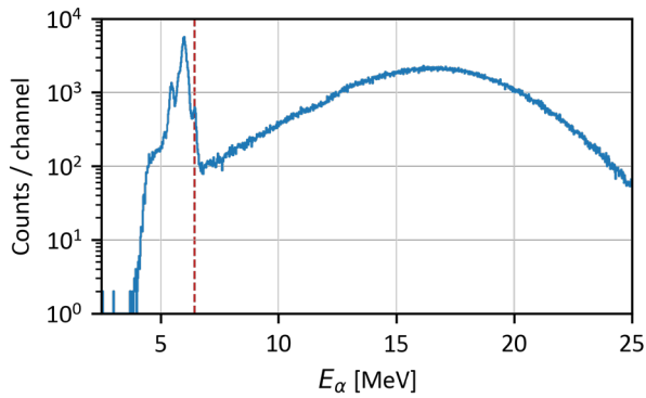
Figure 3: Background-reduced spectrum of implantation events and \alpha -decays of combined runs ( t_{\text{exp}} = 180 min) with a 3.8\text{ }\mu\text{m} -thick Al degrader foil; the peak on the high-energy shoulder at approximately 6.45 MeV indicates the presence of ^{178}\text{Hg} (red dashed line).
