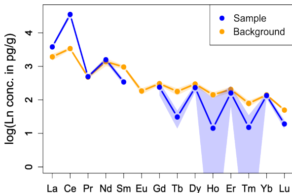
Figure 2: The lanthanoid pattern in the uranyl nitrate sample (blue) together with the method background (yellow).
