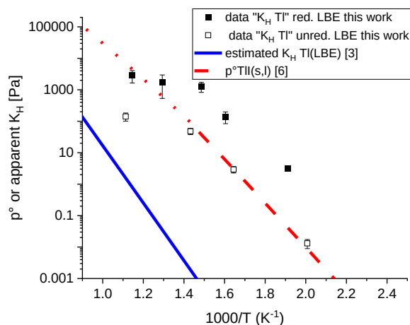
Figure 4: apparent Henry constant of TI in unreduced (open squares) and reduced LBE (filled squares) containing non-carrier-added amounts of iodine, measured in purified helium gas at a flow of 100 ml/min.
