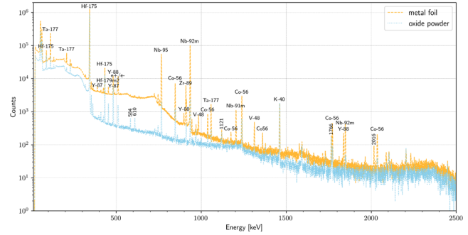
Figure 6: Spectra of the 24 h measurement for both samples.
