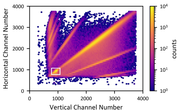
Figure 2: Example plot of the original data (events in all pixels) of one run with the linear center line as the region of consistent energy signals in both detectors (the framed white rectangle marks the region of the aimed at \alpha -spectrum).
