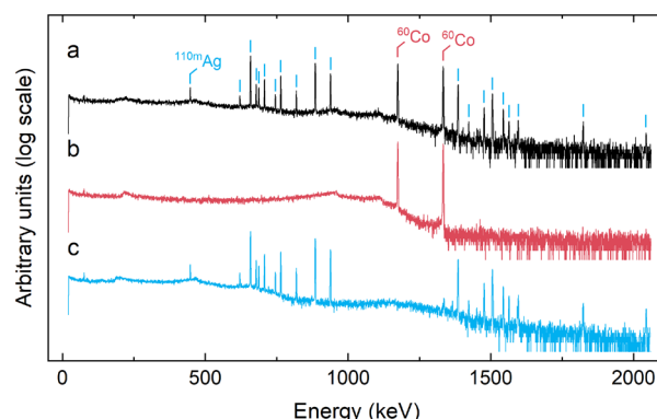
Figure 4: \gamma -spectra of a solution containing carrier-added ^{110m}\text{Ag} and ^{60}\text{Co} in 1M HNO 3 (a) before, and after (b) the separation of Co and (c) the recovery of Ag by flow electrolysis. ^{110m}\text{Ag} -related lines are marked in blue, and ^{60}\text{Co} -related lines in red.
