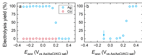
Figure 2: Flow electrolysis yield as function of E_{app} for (a) the electrodeposition of a sample containing 10 µg Ag and Co in 1M HNO 3 (10 ppm of Ag and Co) and (b) the anodic dissolution of 10 µg Ag in 1M HNO 3 ; in (b), Ag was electrodeposited on the WE at the potential indicated by the arrow before anodic stripping. Error smaller than the displayed data points.
