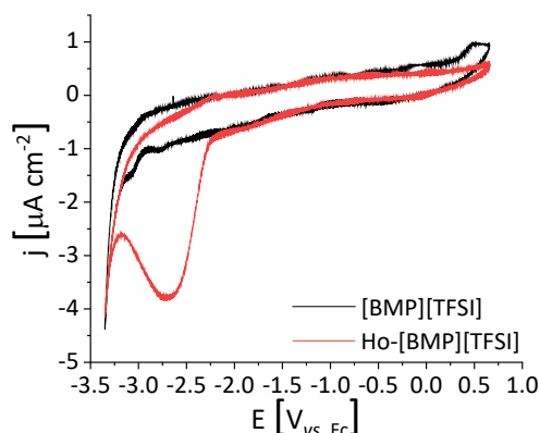
Figure 1: Second cycle of the CV responses recorded at 100 \text{ mV s}^{-1} for pure [BMP][TFSI] (black) and Ho-[BMP][TFSI] (red).
