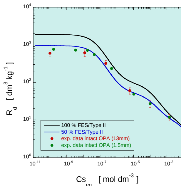
Fig. 7.1: Sorption of ^{134}\text{Cs}^{+} on intact OPA from Mont Terri in equilibrium with artificial pore water. The black solid line represents the modelling of the sorption data on crushed OPA. The blue solid line represents the modeling of the data measured on intact OPA. To model the data on intact OPA, the site capacities of FES and type II sites were reduced by a factor of two.
