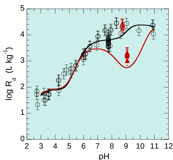
Fig. 4.7: Effect of \text{NaHCO}_3 on Ni sorption edges on Na-illite in the absence (O; \Delta ) and presence ( \blacktriangle ) of 100 mM \text{NaHCO}_3 .
