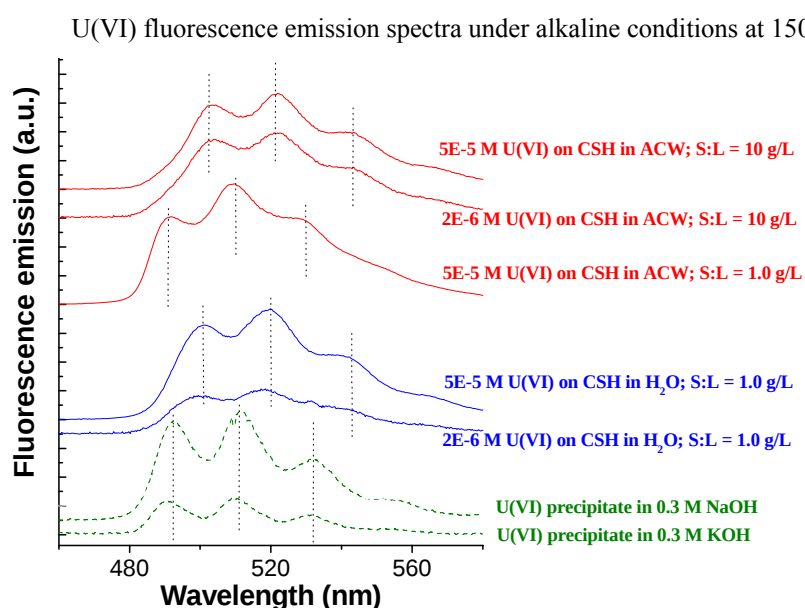
Fig. 5.3: TRLFS spectra of U(VI) precipitates and U(VI) sorbed on CSH phases under alkaline conditions in alkali-free solution (“in \text{H}_2\text{O} ”) and in ACW. In the latter samples the solid-to-liquid ratio (S:L) was varied.
