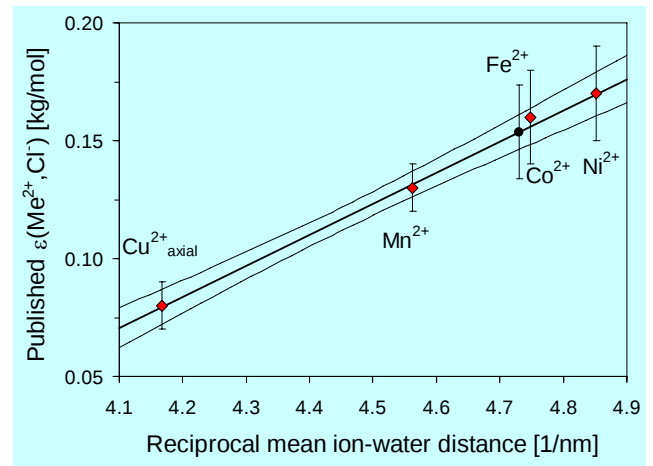
Fig. 2.2: Weighted linear regression of published SIT coefficients \epsilon(\text{Me}^{2+}, \text{Cl}^-) against the reciprocal ion-water distance from MARCUS (1988). The confidence interval suggests an uncertainty below \pm 0.02 [kg/mol].
