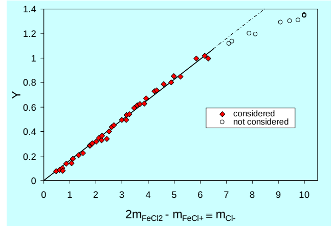
Fig. 2.1: Determination of \epsilon_{(\text{Fe}^{2+}, \text{Cl}^-)} from osmotic data in the \text{FeCl}_2\text{-H}_2\text{O} system at 25 °C under the assumption that \log_{10}\beta_1^0(\text{FeCl}^+) = (-0.111 \pm 0.027) as derived from HEINRICH & SEWARD (1990). Experimental systems producing chloride molalities above \sim 6m were not considered (empty symbols). \epsilon_{(\text{Fe}^{2+}, \text{Cl}^-)} = (0.165 \pm 0.002) and \epsilon_{(\text{FeCl}^+, \text{Cl}^-)} = (0.370 \pm 0.002) [kg/mol] produced the excellent fit shown ( r^2 = 0.994 ).
