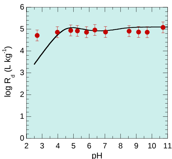
Fig. 4.2: Sorption edge for ^{233}\text{Pa(V)} on Na-SWy-1 in 0.1 M \text{NaClO}_4 . The continuous curve is the calculated Pa(V) sorption edge using the 2SPNE SC/CE model.
