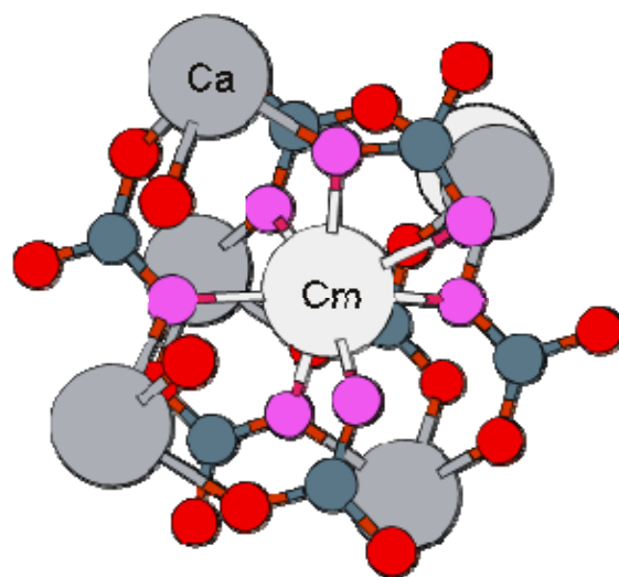
Fig. 3.3: The structure of \text{Cm}^{3+} in calcite formed by the substitution mechanism given in equation (1). The seven oxygen sites building the first coordination shell of the \text{Cm}^{3+} ion are marked in pink.
