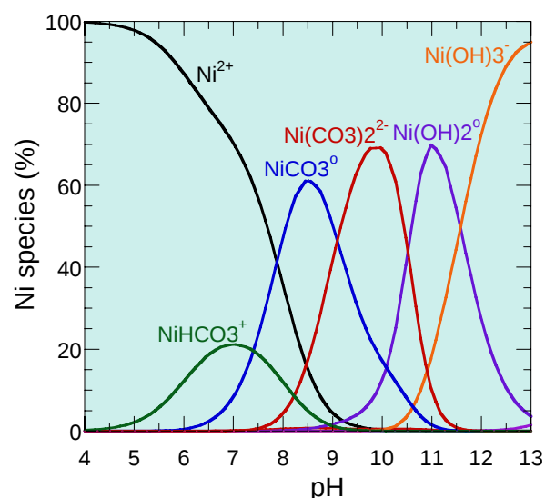
Fig. 4.6: The Ni aqueous speciation in 0.1 M \text{NaClO}_4 as a function of pH. The total inorganic carbon concentration is 100 mM.
