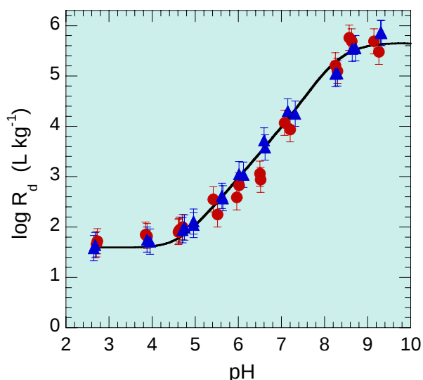
Fig. 4.1: Sorption edges for ^{241}\text{Am(III)} (●) and ^{152}\text{Eu(III)} (▲) on Ca-SWy-1 in 0.066 M \text{CaCl}_2 . The continuous curve is the calculated Am(III) sorption edge using the 2SPNE SC/CE model.
