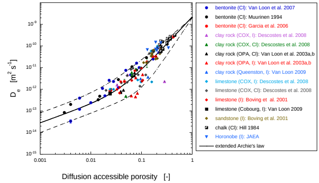
Fig. 7.2: Extended Archie's Law (solid line) describing the relationship between the diffusion accessible porosity and the effective diffusion coefficient for anions.
