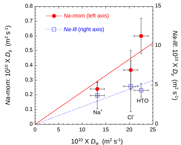
Fig. 7.3: Normalised pore diffusion coefficients ( D_p ) for the diffusion of HTO, 22 Na and 36 Cl - in Na-montmorillonite (Na-mom) and Na-illite (Na-ill) in comparison with the respective D_w values.
