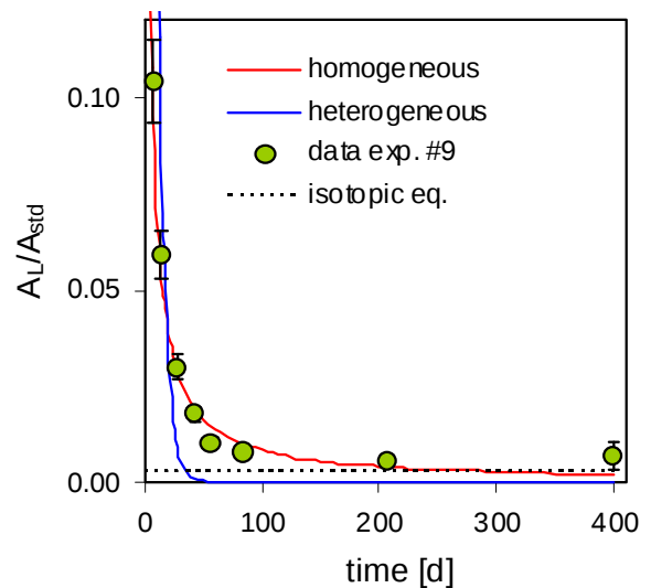
Fig. 2.4: Ratio of ^{133}\text{Ba} activity in solution ( A_L ) to total added activity ( A_{\text{std}} ) as a function of reaction time for barite in pure water, compared with model calculations for homogeneous (red continuous line) and heterogeneous incorporation (blue continuous line). The broken line indicates isotopic equilibrium between bulk solid and aqueous solution.
