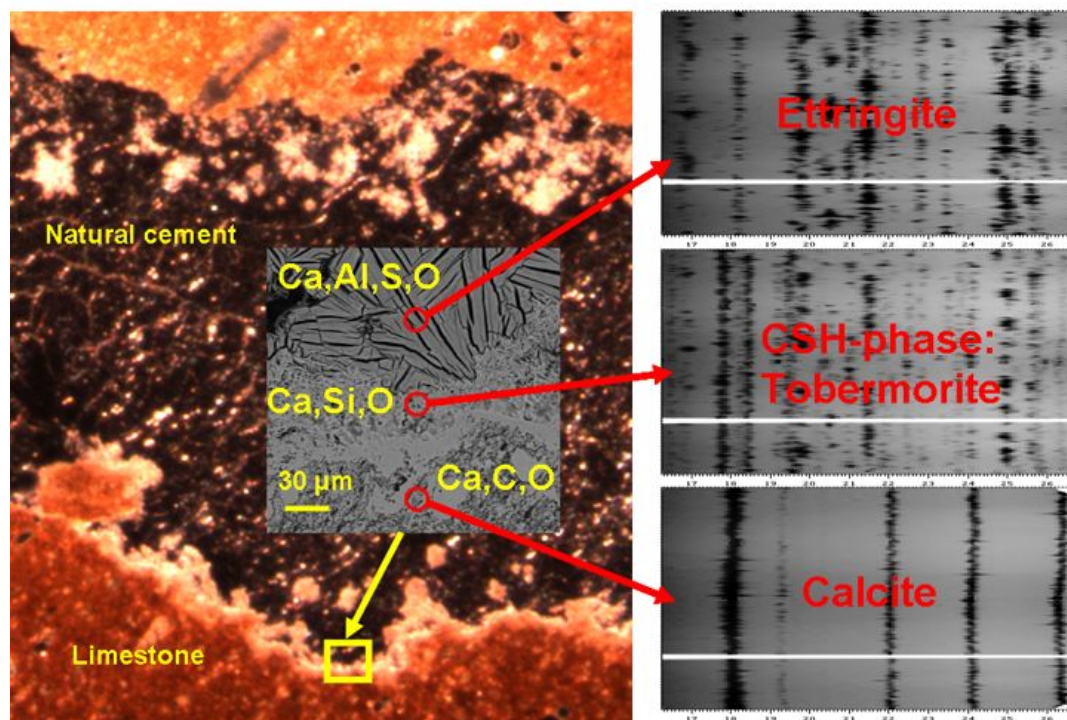
Fig. 5.7: Identification of major crystalline components (right) across the interface between the cementitious in-fill (natural cement) and surrounding limestone (left; \lambda = 0.9537\text{\AA} ).
