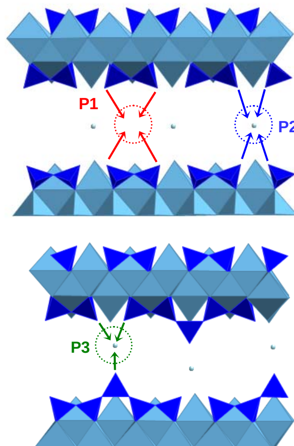
Fig. 5.6: Three possible positions of U(VI) in the interlayer of two different C-S-H structures providing uranophane-like (P1 and P2) and soddyite-like (P3) molecular environments. These structural arrangements represent three out of nine end member stoichiometries.
