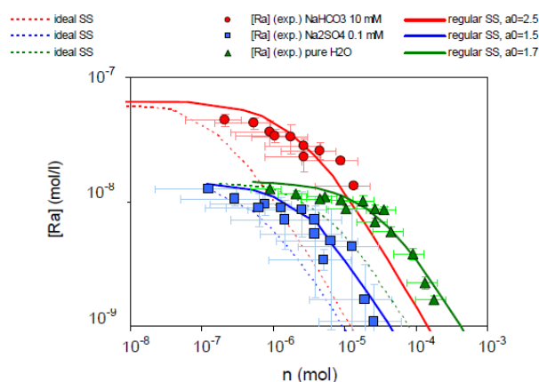
Fig. 2.6: Ra-barite solid solution data compared to GEMS-PSI model calculations. Broken lines: ideal solid solutions. Solid lines: best fits obtained by adjusting the non-ideality parameter a_0 .
