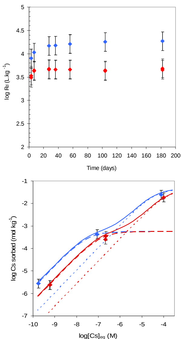
Fig. 4.3: a) Cs sorption kinetics for conditioned Na-IdP (pH ~7, 0.1 M NaClO 4 ) on the FES sites at 25 °C (♦) and 90 °C (♦). b) Cs sorption isotherm after 182 days at 25 °C (♦) and 90 °C (♦). The solid lines are the fit to the data using the parameter values given in Table 4.1. The dashed and dotted lines are the contributions made by FES and type II sites to the overall sorption of Cs, respectively.
