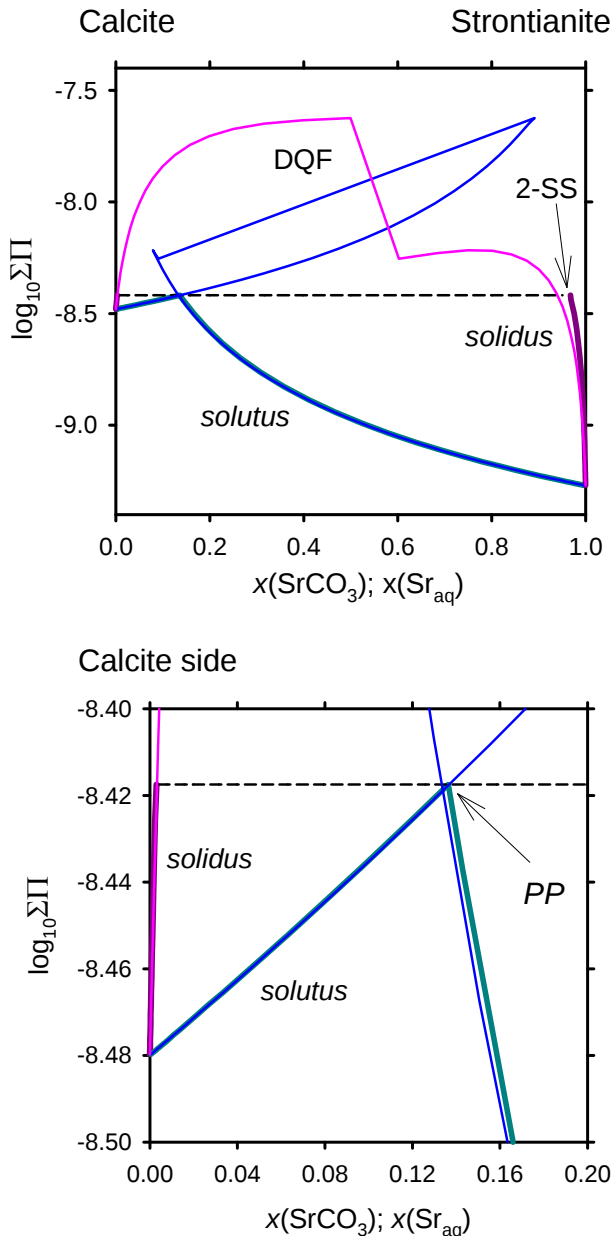
Fig. 2.3: Analogue of the Lippmann diagram for two (\text{Ca,Sr})\text{CO}_3 phases, one with the calcite structure (left thick lines, calcite incorporating some Sr) and one with the aragonite structure (right thick lines, strontianite incorporating some Ca). The thick lines below the dashed horizontal line show the miscibility gap. PP is the peritectic point where the solution is in equilibrium with two solids. A superimposed Lippmann diagram (thin lines) shows the model calculations according to the DQF mixing model for one solid solution phase with calcite and strontianite end members. The thin lines above the dashed horizontal line represent metastable solid solutions. The step in the red line indicates the structural transition of the solid solution phase from the calcite to the aragonite structure.
