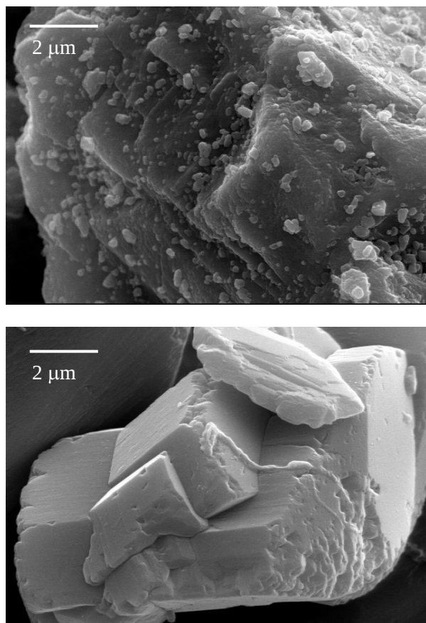
Fig. 2.5: SEM images of the barite used for the ^{133}\text{Ba} and ^{226}\text{Ra} tracer experiments before (top) and after 18 months reaction time in deionised water (bottom). The small nanometre-sized barite particles on top of the crystal surfaces of the pristine barite disappeared during the recrystallization process. In addition, surface roughness decreased and the crystal habitus became idiomorphic.
