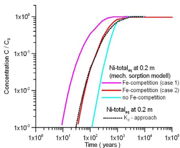
Fig. 3.6: Ni breakthrough curves at x=0.2 m from the source in the bentonite calculated for different Fe solubility limits and different sorption model setups (sorption competition vs. no-competition) compared to the breakthroughs predicted by a K_d approach. Ni boundary concentration ( C_0 ) was 10^{-5} M, initial Ni background was assumed to be 10^{-10} M. Case 1: Fe(II) concentration in the porewater was limited by the solubility of siderite. Case 2: the equilibrium Fe(II) concentration in the porewater was set to be 10 times lower than the solubility of siderite.
