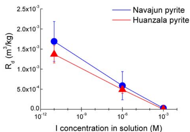
Fig. 2.7: R_d values of I sorption onto pyrite after 7 days reaction time.
