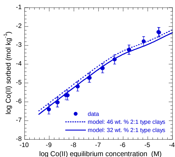
Fig. 4.2: Sorption of Co(II) on Opalinus Clay: the symbols are measured data, the lines are the model prediction using the "bottom up" approach.
