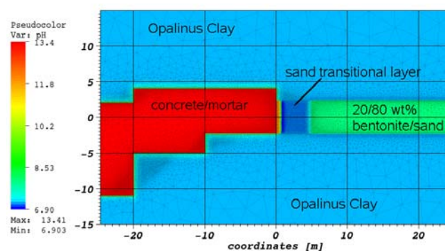
Fig. 3.4: Migration of a high pH-plume in the near field of a fully saturated LLW-repository after 25 years. Preliminary calculations for a diffusive transport scenario. Colour scheme indicates pH distribution.
