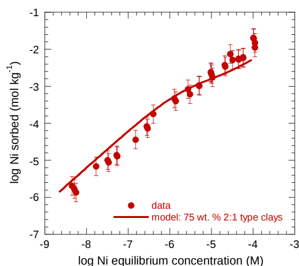
Fig. 4.1: Sorption of Ni(II) on MX-80 bentonite: the symbols are measured data, the solid line is the model prediction using the "bottom up" approach.
