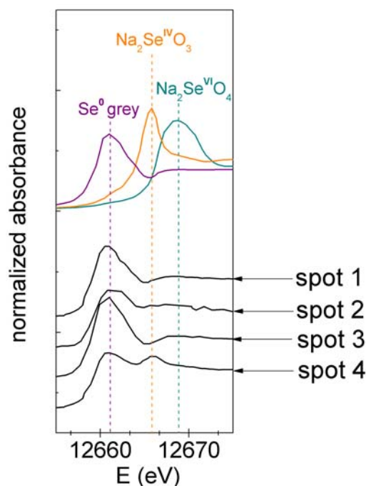
Fig. 2.9: Se K-edge \mu -XANES of the selected spots, compared to the white line positions for the oxidation states 0, IV and VI as defined by reference compounds.
