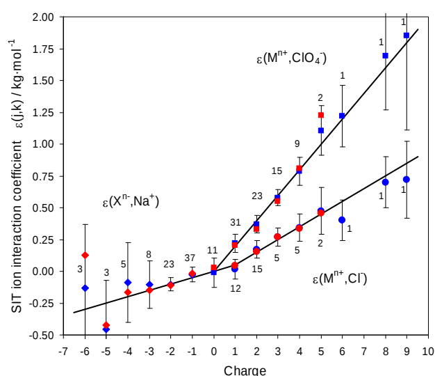
Fig. 2.1: Correlation of SIT interaction parameters with charge only. Blue symbols with error bars represent un-weighted means where the uncertainty is based on the dispersion of the data points. Red symbols represent weighted means, their uncertainties are always \pm 0.02 or less, i.e. within the size of the red symbols. The number of data points used to calculate the means are given in the figure. In some cases there is only one measured data point, and the given experimental error is indicated. In all cases the uncertainty is estimated on the 95% confidence level. Black solid lines show the finally selected “default values” of SIT interaction parameters.
