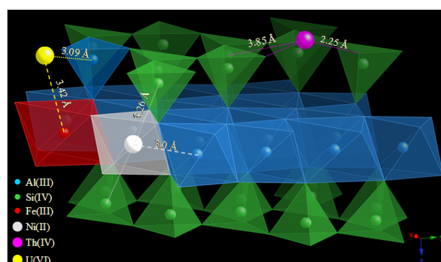
Fig. 4.4: Specific strong sorption site types for Ni(II), Th(IV) and U(VI) on montmorillonite as determined by EXAFS.
