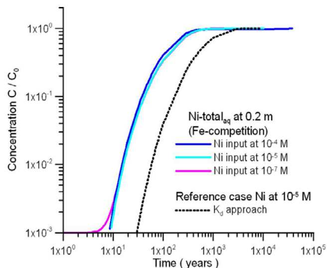
Fig. 3.5: Ni breakthrough at x=0.2 m from the source in the bentonite calculated for different input Ni concentration levels ( C_0=10^{-4} M, 10^{-5} M, and 10^{-7} M) using the mechanistic sorption model and the numerical K_d approach. The Fe(II) concentration in porewater is given by the siderite solubility.
