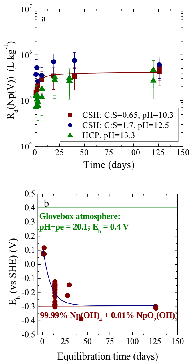
Fig. 5.1: Np(V) sorption kinetics on C-S-H phases with different C:S ratios under alkali ion free conditions and in artificial cement porewater (ACW) at pH = 13.3. a) R_d values for Np(V) sorption onto two C-S-H phases and on HCP. b) Changes in the redox potentials of Np(V) – C-S-H suspensions in ACW at pH 13.3 with increasing equilibration time.
