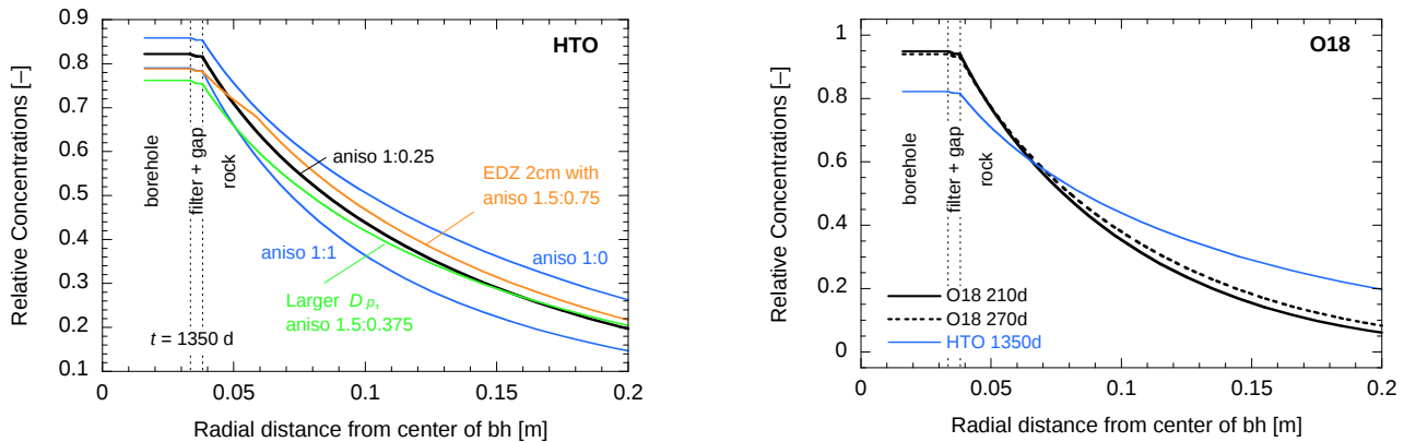
Fig. 3.2: Left: Predicted porewater concentration profiles for HTO tracer after 1350 d (i.e., the end of 2009). The black lines represent the reference case (anisotropy ratio of 1:0.25 and other parameters estimated from earlier experiments). The coloured lines represent the results for alternative model parameters (different anisotropy ratio, larger pore diffusion coefficient, presence of a disturbed zone). Right: Predicted porewater concentration profiles for ^{18}\text{O} after 210 d and 270 d (i.e., for the originally foreseen time span for the over-coring, at 1.11.2009 and 31.12.2009, respectively), using parameters from previous experiments. The predicted profile for HTO tracer is shown for comparison.
