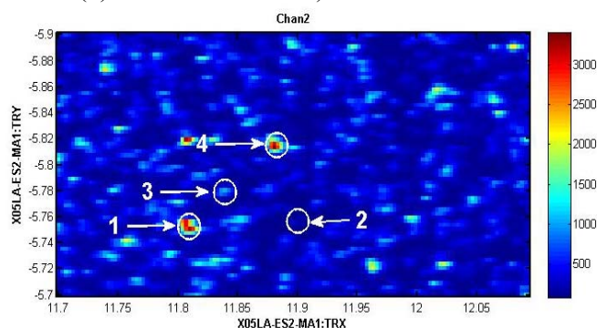
Fig. 2.8: Color coded micro-XRF map of the Se-K \alpha signal for a polished pyrite chip reacted during two months with Na_2SeO_3 under anoxic conditions. Selected analyzed \mu -XANES spots are labelled 1 to 4.
