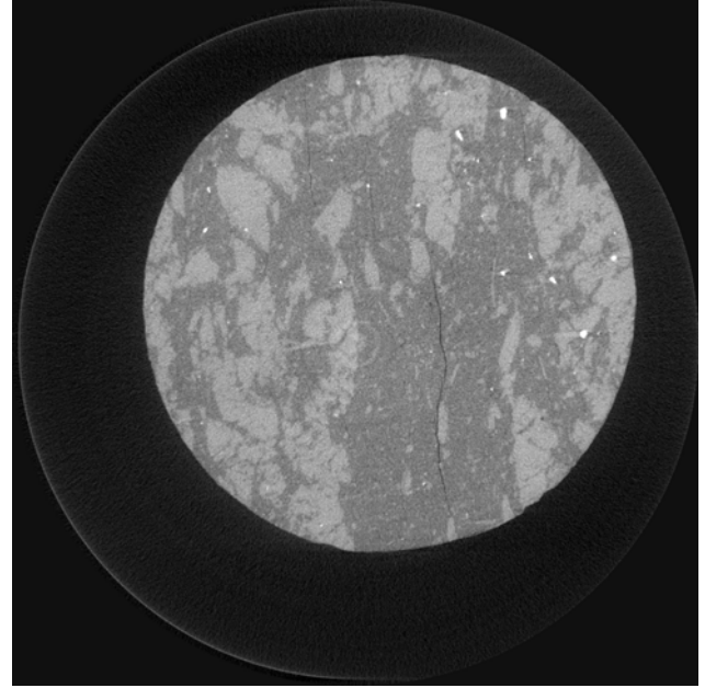
Fig. 3.10a: Horizontal slice through a cylindrical sample of Opalinus Clay from Mont Terri (sample diameter: 3 mm). The measurements were performed at the PSI TOMCAT beam line. Two major mineral domains, and some small-scale impurities, are clearly resolved. Light-grey is clay matrix. Dark-grey is calcite ( \text{CaCO}_3 ). Bright spots are high density inclusions of Fe-oxides (to be confirmed).
