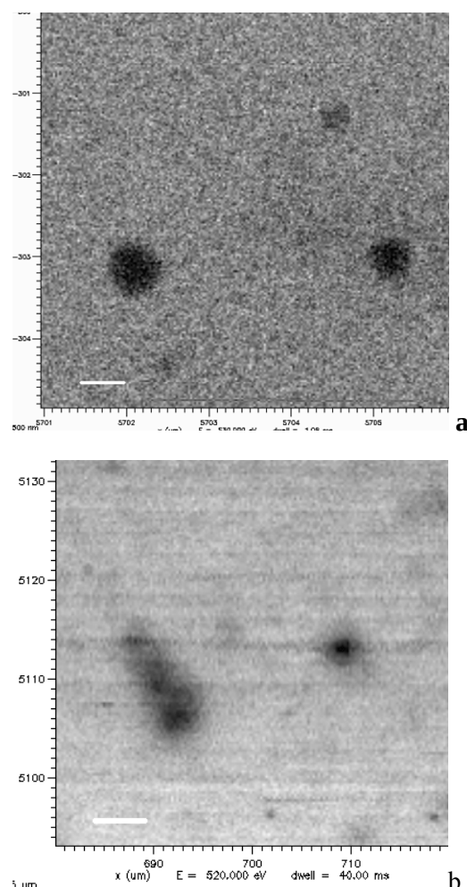
Fig. 6.2: X-ray micrograph of montmorillonite clay aggregate in 0.001 M (a), and in 0.1 M (b) NaCl. Conditions: bar scale 500 nm (a), 1000 nm (b). Note the heterogeneous aggregate structure in the NaCl concentrated suspension.
