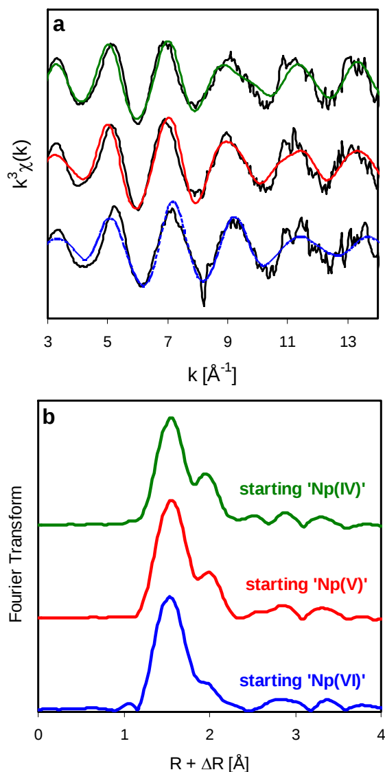
Fig. 5.2: a) EXAFS spectra (experimental and modelled) and b) Fourier-transformed EXAFS for Np(IV), Np(V) and Np(VI) starting valencies sorbed on C-S-H (C:S = 1.0).
