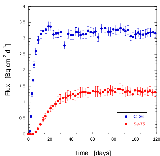
Fig. 7.1: Diffusion (flux vs. time) of ^{36}\text{Cl}^- and ^{75}\text{SeO}_4^{2-} in Opalinus Clay. Diffusion of ^{75}\text{SeO}_4^{2-} is slower than ^{36}\text{Cl}^- and can be explained by the factor of two lower diffusion coefficient of ^{75}\text{SeO}_4^{2-} in water (LI & GREGORY, 1974; D_{w,\text{Cl}} = 2.03 \times 10^{-9} \text{ m}^2 \text{ s}^{-1} ; D_{w,\text{Se}} = 9.46 \times 10^{-10} \text{ m}^2 \text{ s}^{-1} ).
