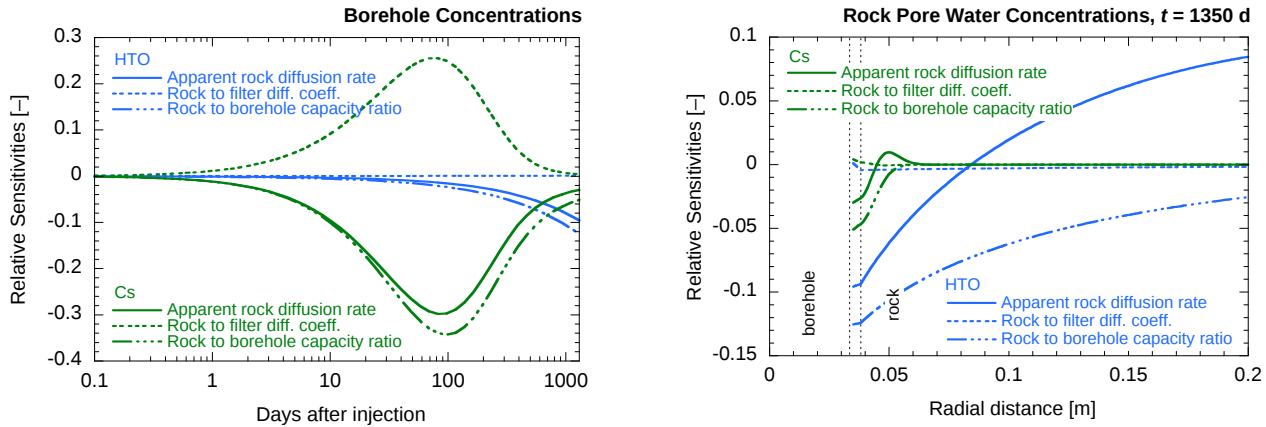
Fig. 3.1: Relative sensitivities of HTO and Cs concentrations in the borehole (left) and in the porewater (right) to three lumped parameters (apparent diffusion ratio in the rock, ratio of rock to filter effective diffusion coefficient, and ratio of rock to borehole capacity).
