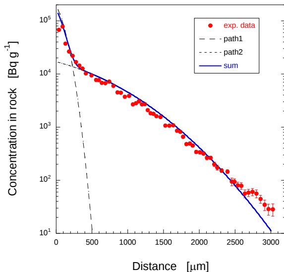
Fig. 3.9: Measured ^{60}\text{Co} distribution in Opalinus Clay from the Mont Terri test site after 50 days of in-diffusion. Such a distribution cannot be explained by a single porous medium transport model. The best fit shown in the figure was obtained using a dual porosity concept. (Figure taken from VAN LOON & MÜLLER, in prep.).
