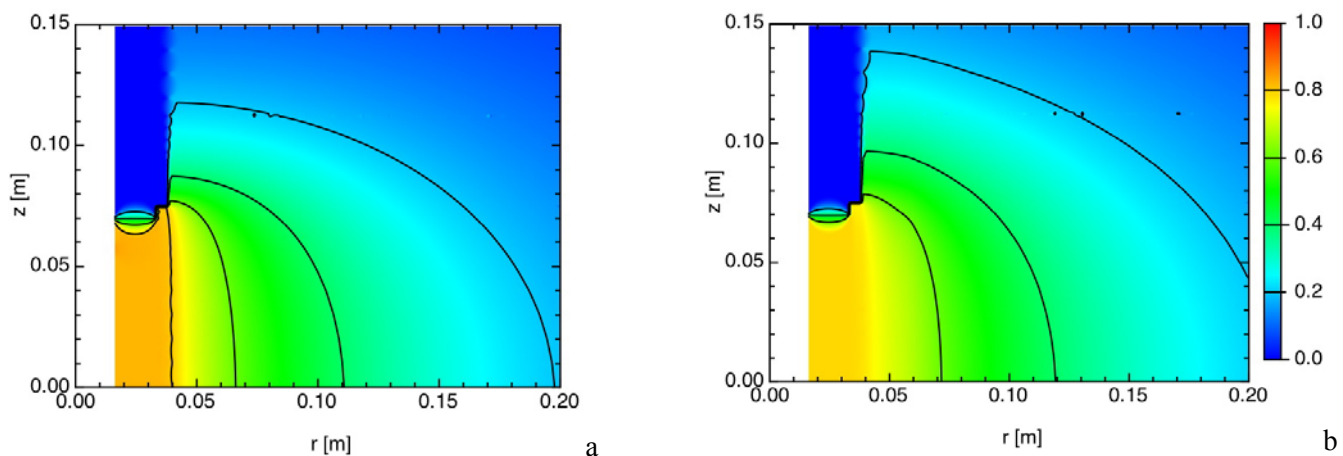
Fig. 3.3: Contour plots of the simulated porewater concentrations for HTO tracer (relative units) after 1350 d (i.e. at the end of 2009). (a) Reference case (anisotropy ratio of 1:0.25, parameters estimated from earlier experiments), (b) case with a 2-cm borehole disturbed zone (EDZ) with larger diffusion coefficients.
