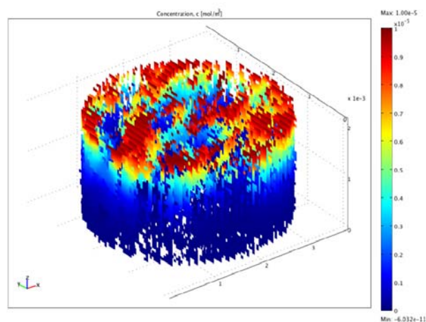
Fig. 3.11: Computed solute concentration distribution profile through the clay fraction of an Opalinus Clay sample from Mont Terri (sample diameter is 3 mm, see Fig. 3.10). The red to blue colour map indicates high and low solute concentrations, respectively. Non-uniform tracer migration through the sample is a consequence of the microscopic heterogeneities in the rock. Interstitial “void space” corresponds to the mineral phases impermeable for the solute transport.
