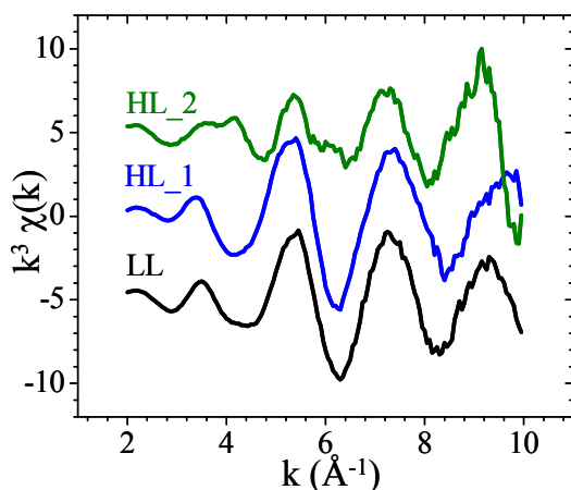
Fig. 5.4: k^3 -weighed EXAFS spectra of the main components obtained with PCA. At low U(VI) loading (LL) all spectra correspond to the spectrum of one U(VI) species. At high U(VI) loading all composite spectra collected at the different U(VI) spots contained two U(VI) species designated as HL_1 and HL_2 species. K-range for data analysis was taken between 2 and 10 Å.
