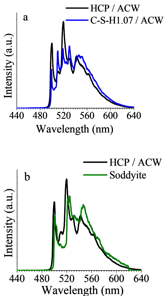
Fig. 5.5: Emission spectra a) for U(VI) sorbed onto HCP in ACW and U(VI) sorbed onto C-S-H (C:S = 1.07) in ACW and b) U(VI) sorbed onto HCP in ACW and soddyite. Measurements: (M)OPO laser system at excitation wavelength of 500 nm and samples at 4 K.
