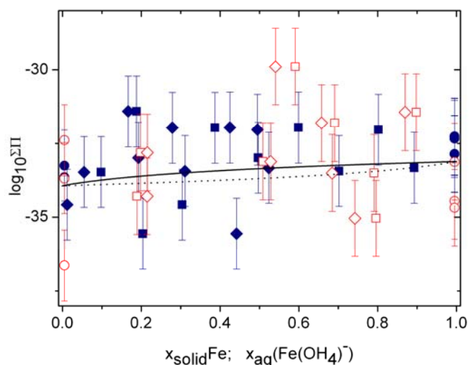
Fig. 2.2: Lippmann solubility diagram of the hydrotalcite – pyroaurite solid solution system at 25°C. The solid line represents the solidus, the mole fraction of Fe in the solid, whereas the dotted line represents the solutus, the corresponding mole fraction of Fe in the solution.
