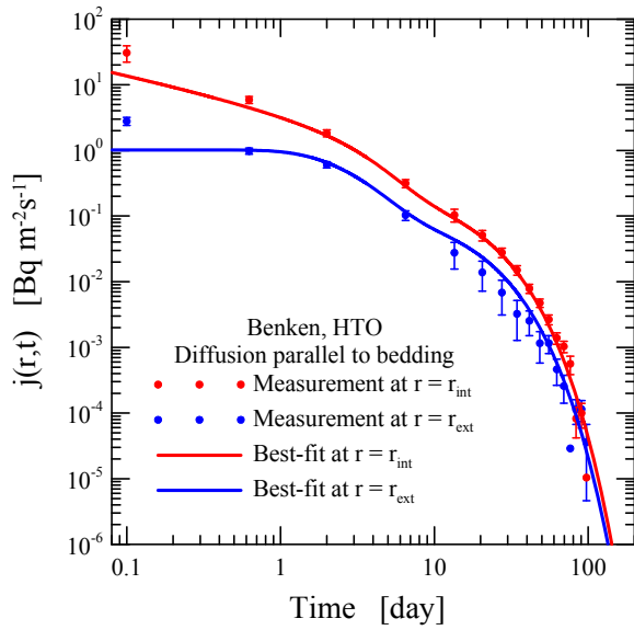
Fig. 3.8: Measured diffusive flux data versus time for tritiated water (HTO) using a hollow cylinder of Opalinus Clay from Benken (Switzerland). Transport of the tracer takes place parallel to the fabric. A second preferential transport pathway accessible for HTO is evident from the bi-modal tracer breakthrough, which cannot be explained by a single porosity model. The best fit was obtained using a dual porosity model. (Figure taken from VAN LOON & JAKOB, 2005).
