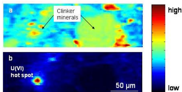
Fig. 5.3: XRF map recorded at the microXAS beamline, a) Ca and b) U distribution in U(VI) doped compact hardened cement paste (U loading = 2500 ppm).
