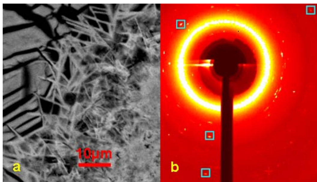
Fig. 5.8: SEM image of a) micro-crystals of tobermorite and b) diffraction pattern from the selected single-crystals with characteristic reflections (squares).
