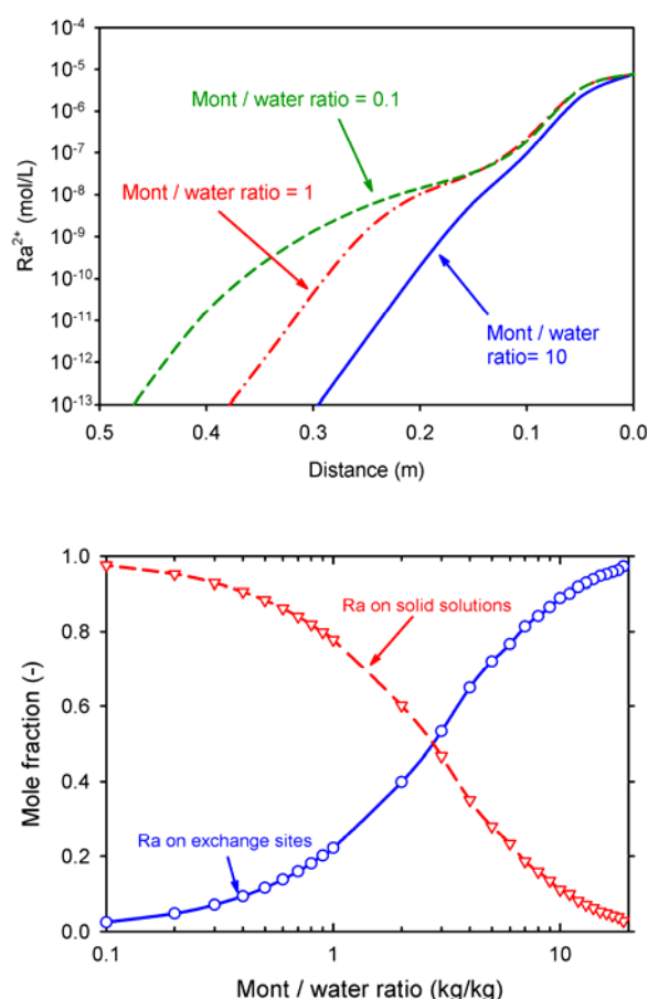
Fig. 3.7: Top: Aqueous phase Ra profile after 1000 years for different Clay water ratios. Bottom: Partitioning of Ra between sulphate solid solutions and Clay cation exchange sorption sites in montmorillonite as function of the montmorillonite-water ratio. Montmorillonite-water mass ratios 1.0 and 10 kg/kg correspond to sand-bentonite mixtures and highly compacted bentonite, respectively.
