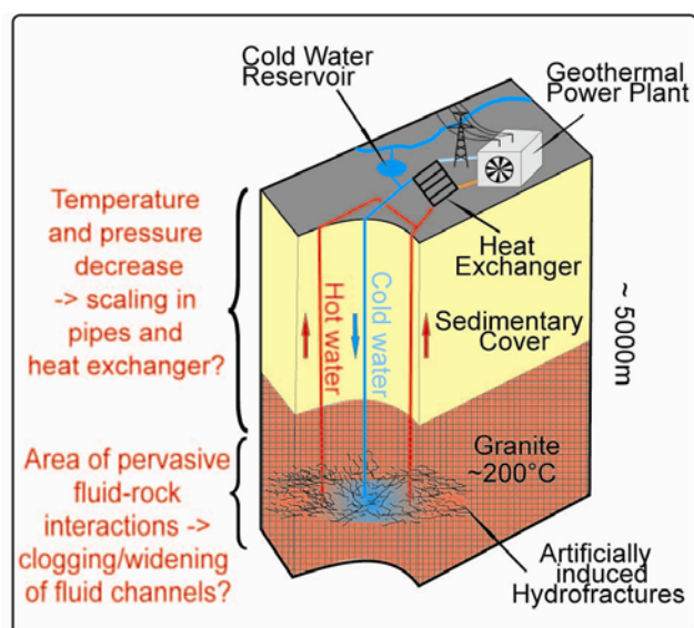
Fig. 3.13: A simplified sketch of a typical Hot-Dry-Rock-EGS. Cold water from a reservoir is pumped into the crystalline basement which is used as a heat source. Heated water is transported upwards to the heat exchanger used for house-heating or for electricity generation in a geothermal power plant. To optimize the power yield efficiency, and prevent scaling of mineral phases in the technical installations, the operating conditions are tuned based on the results of the thermodynamic modelling.
