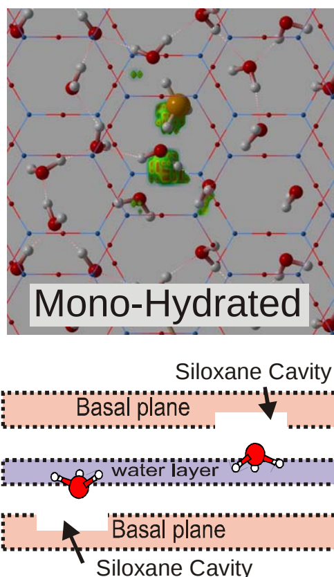
Fig. 3.12: Top: Probability density distribution (green to grey shaded area) of H_3O^+ ion in the interlayer of monohydrated montmorillonite seen in the [001] direction. An instantaneous configuration of the H_3O^+ ion is shown as a large brown sphere. Water molecules are shown as red spheres (oxygen sites) attached to two small gray spheres (hydrogen sites). Upper and lower tetrahedral layers of clay sheet are shown as tiny red (oxygen) and blue (silica) spheres attached in a typical pseudo-hexagonal framework. Bottom: a schematic view of a preferential orientation of H_3O^+ in a monohydrated montmorillonite.
