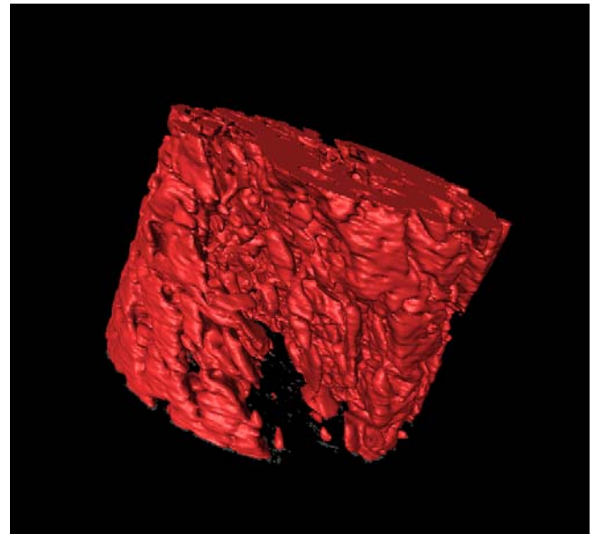
Fig. 3.10b: Reconstructed 3D clay domain of the Opalinus Clay sample based on individual 2D-slices. The extracted clay mineral distributions were used in the subsequent transport modelling.
