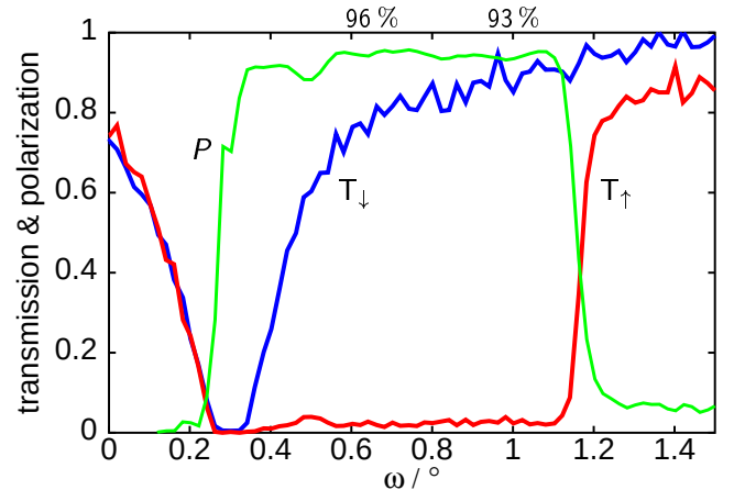
Fig.3: Transmission of spin up ( T_{\uparrow} ) and spin down ( T_{\downarrow} ) neutrons through a Fe 89 Co 11 / Si, m = 2.3 supermirror with 299 layers in total. The polarizer was measured in a magnetic field of 300 G. \omega gives the angle of incidence, the neutron wavelength was \lambda = 4.74 \text{ \AA} . The line denoted P gives the polarizing efficiency.
