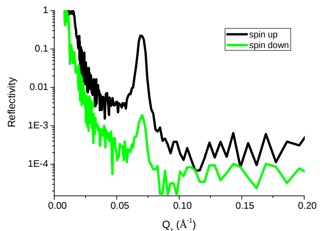
Figure 2: Polarized neutron reflectivity experiments on AMOR. The peak in the green curve is caused by a non-perfect polarizer.
