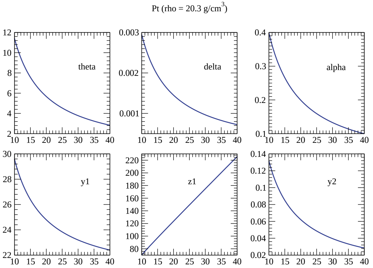
FIG. 4: Optics geometry when using the Pt-stripe of the mirrors. The energy region of interest is 10 to 40 keV.
